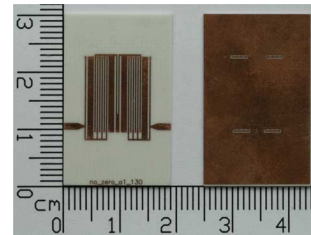
Fig. 4. Top view (left side) and bottom view of the fabricated filter I.
