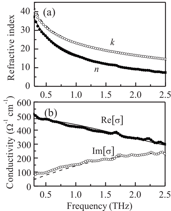
FIG. 1. Real (solid circles) and imaginary (open circles) parts of (a) refractive index and (b) conductivity of the InN film. Solid and dashed lines correspond to the calculated results based on the simple-Drude model. The fitting parameters are listed in Table 1.
