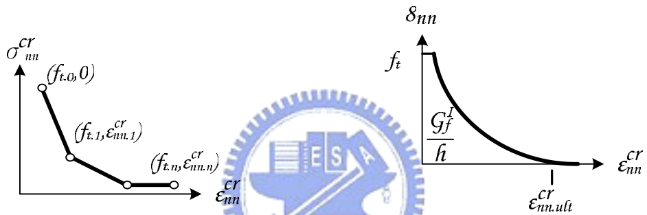
(d) Nonlinear tension softening (Moelands and Reinhardt)
