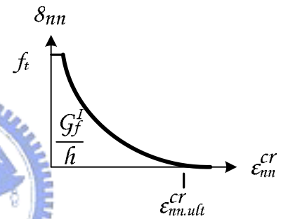
(d) Nonlinear tension softening (Moelands and Reinhardt)
