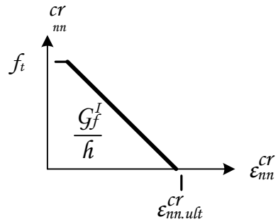
(b) Linear tension softening
