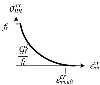
(e) Nonlinear tension softening (Hordijk et al.)
