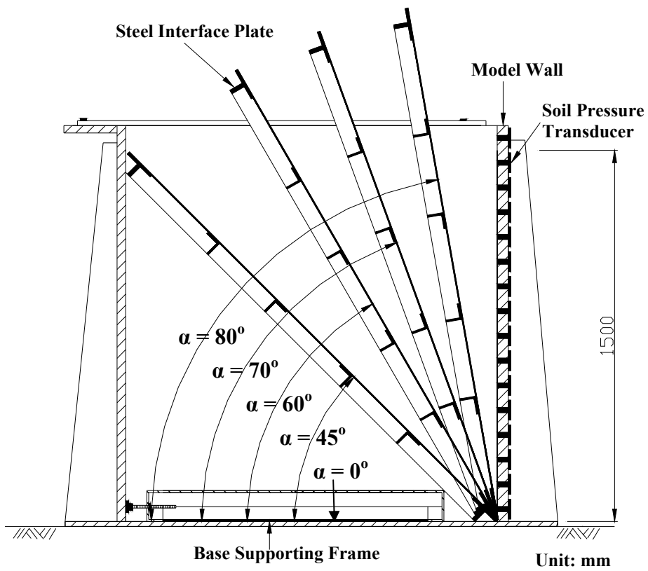
Fig. 1.4. Different interface inclinations
