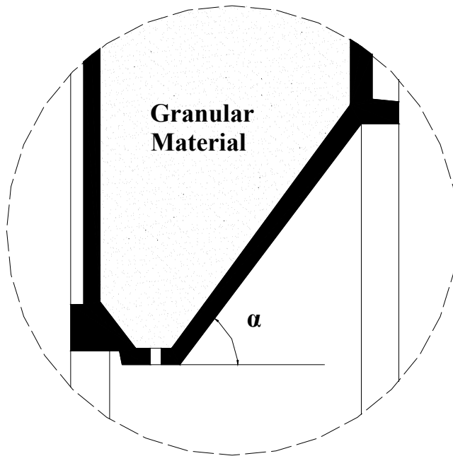
(b) Hopper of the storage silo
