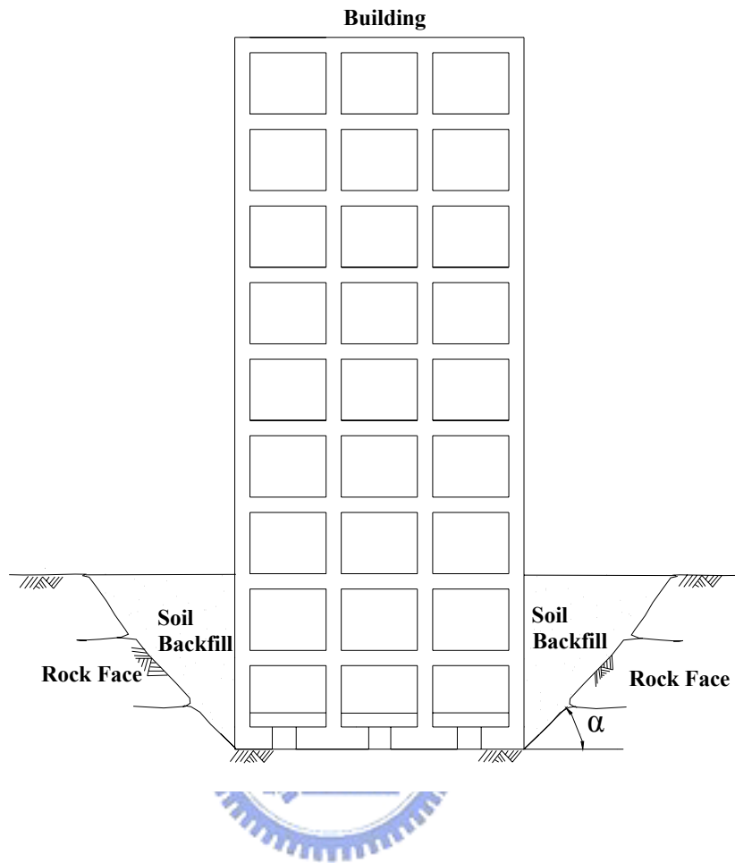
Fig. 1.2. Basement wall near inclined rock faces
