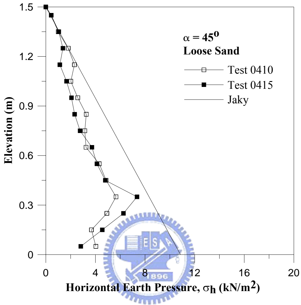
Fig. 6.3. Distribution of lateral earth pressure at \alpha = 45^\circ for loose sand
