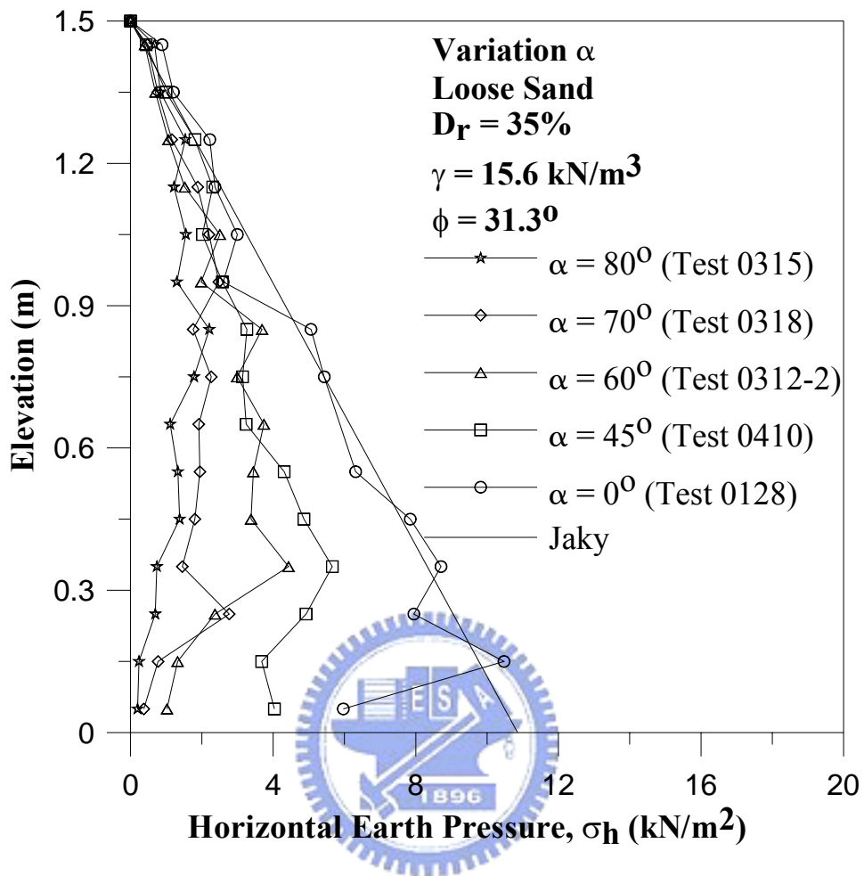
Fig. 6.7. Distribution of lateral earth pressure at various \alpha for loose sand
