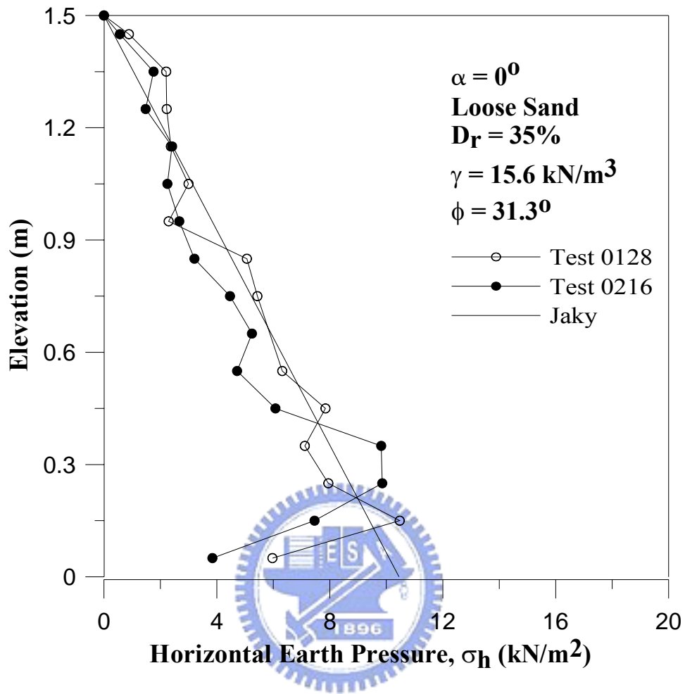
Fig. 6.2. Distribution of lateral earth pressure at \alpha = 0^\circ for loose sand
