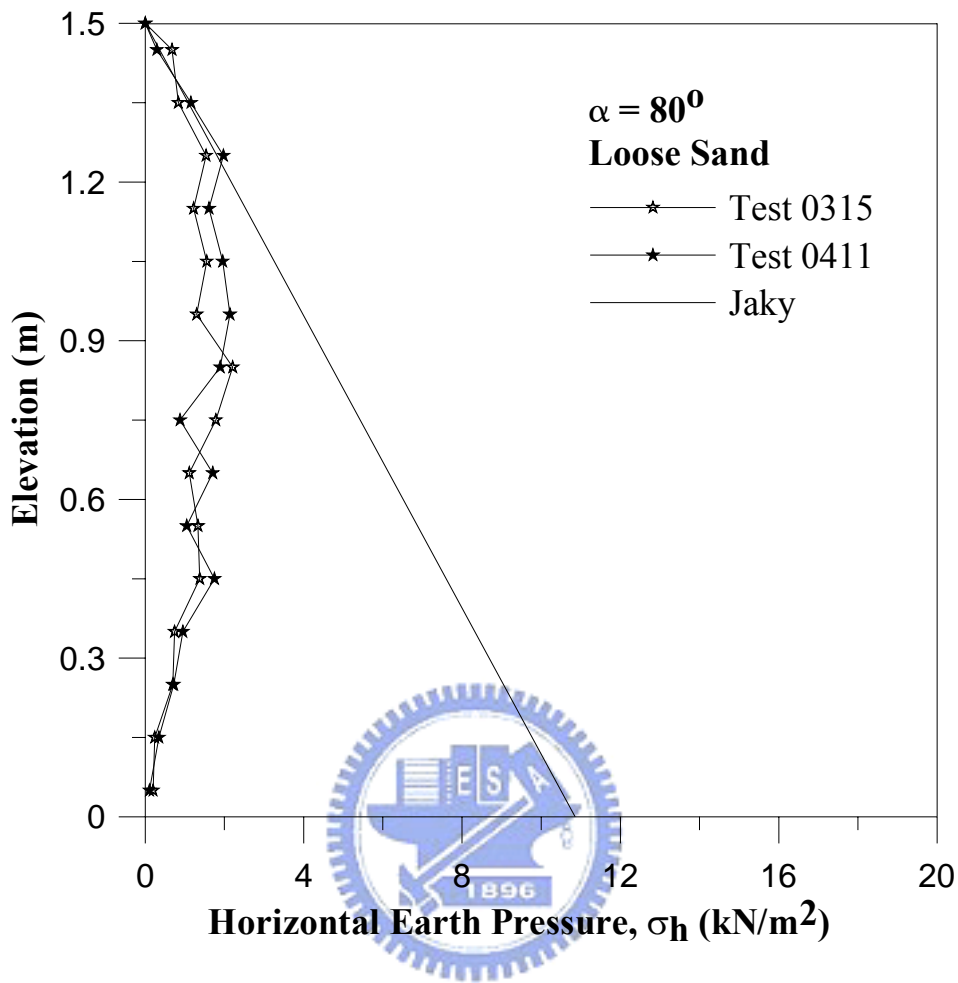
Fig. 6.6. Distribution of lateral earth pressure at \alpha = 80^\circ for loose sand
