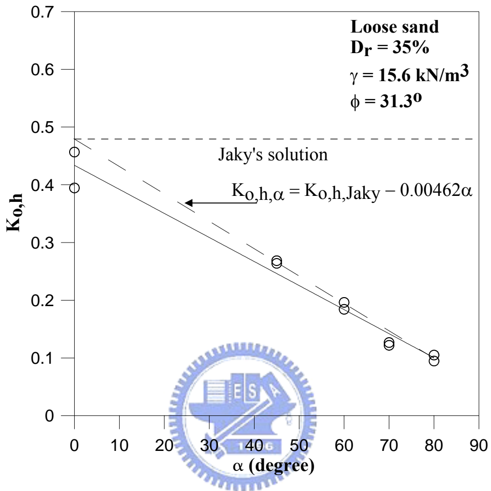
Fig. 6.8. Variation of K_{o,h} at various \alpha for loose sand
