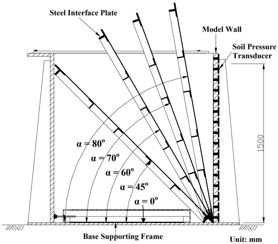
Fig. 6.1. Different interface inclinations
