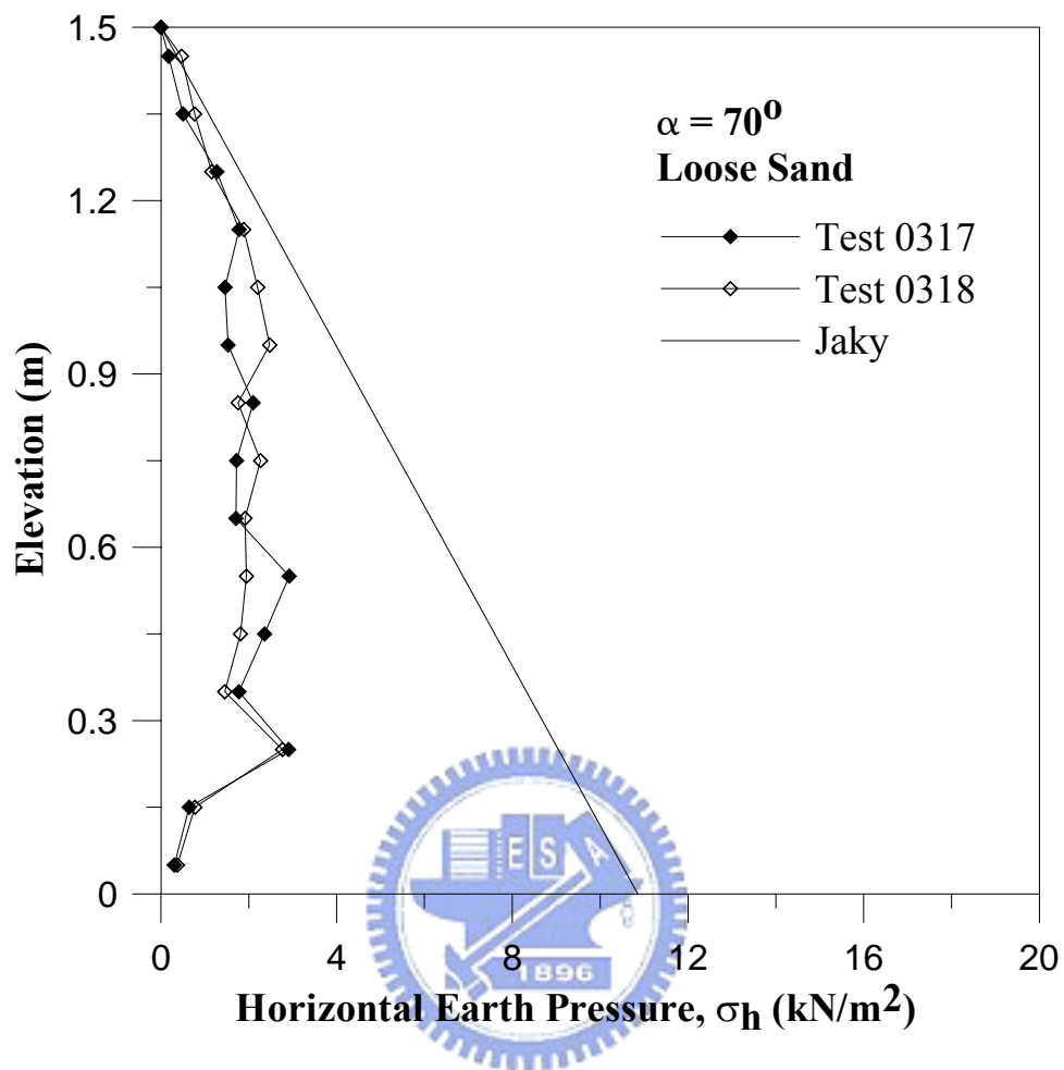
Fig. 6.5. Distribution of lateral earth pressure at \alpha = 70^\circ for loose sand
