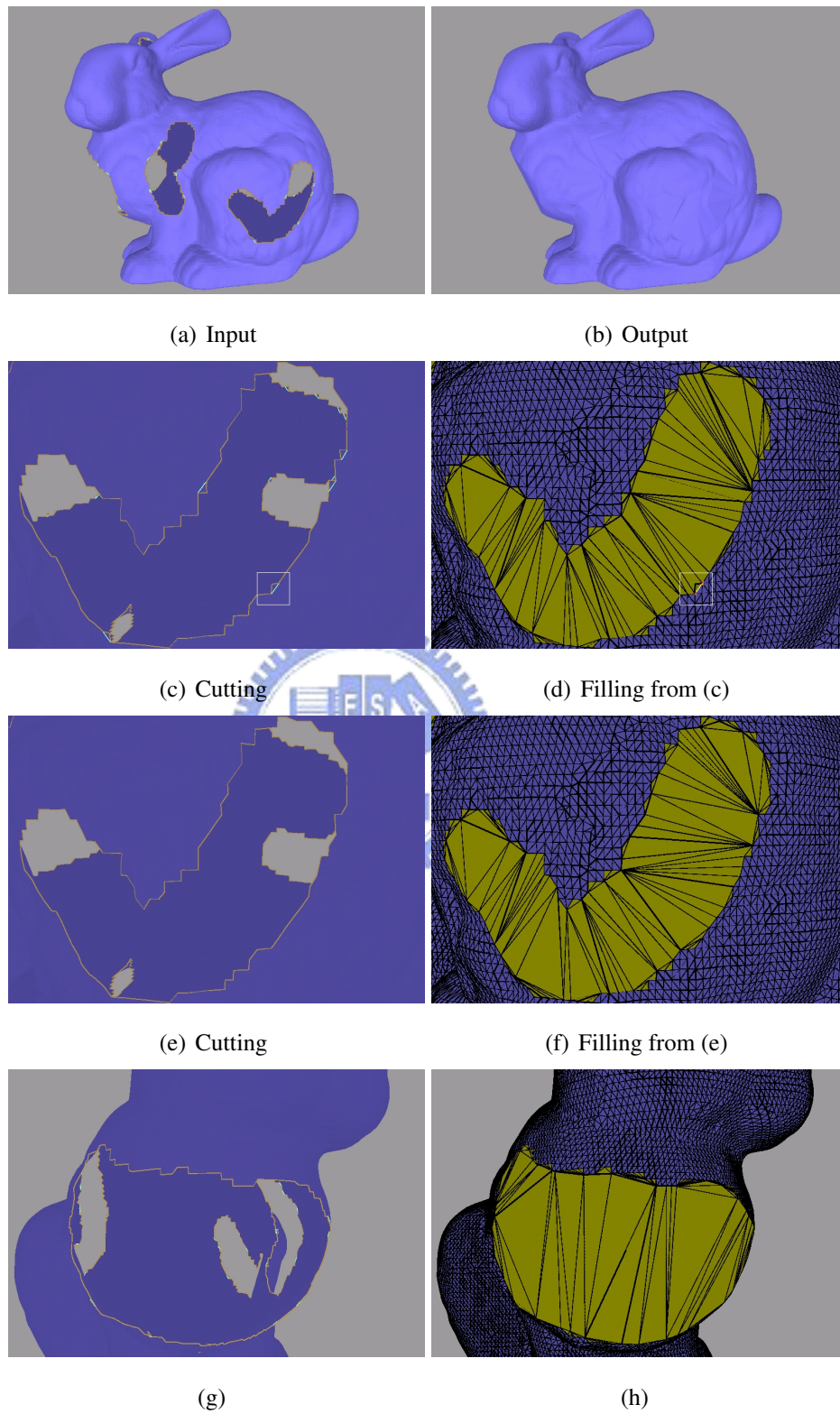
Figure 4.3: Bunny model
