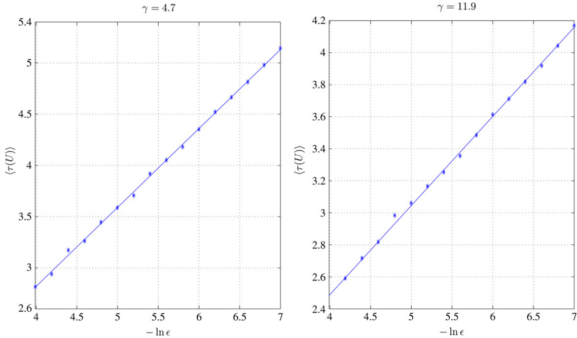
Fig. 3.3. Poincaré recurrences of MLM for \gamma = 4.7 and 11.9 with respect to the slopes 0.77 and 0.57 , respectively. The dispersion of the calculated values of the slopes is about 3\% .
