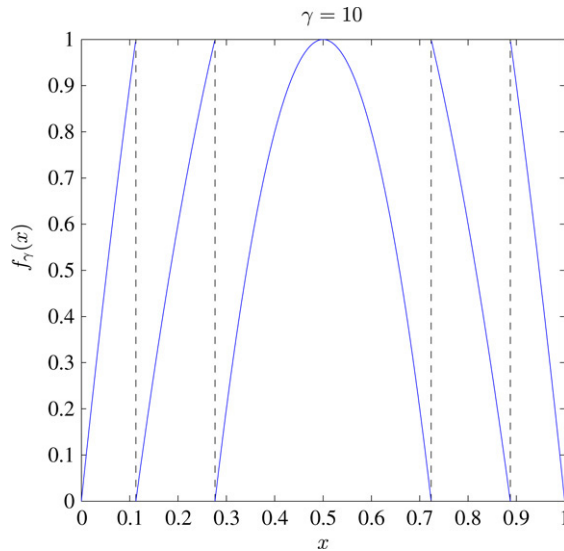
Fig. 2.1. MLM with \gamma = 10 .
