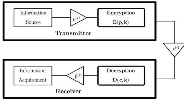
Fig. 5.1. Communication scheme.
