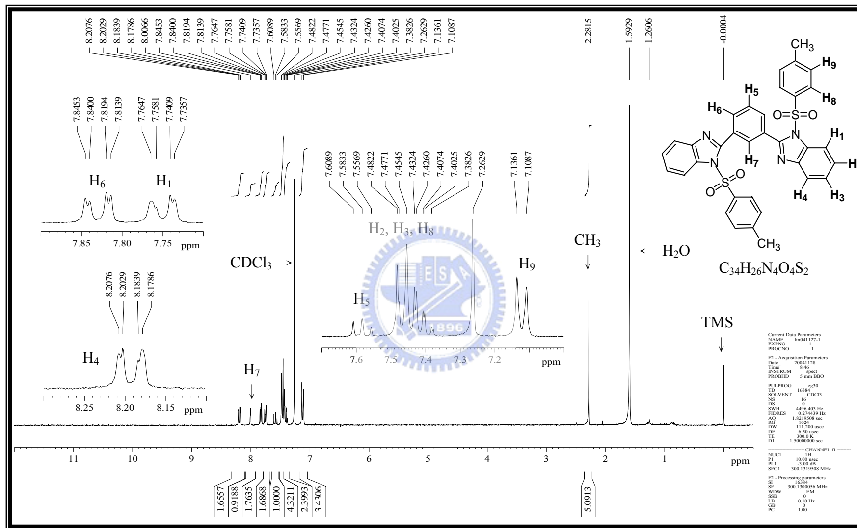
附圖 26 化合物 1-[(4-methylphenyl)sulfonyl]-2-(3-{1-[(4-methylphenyl)sulfonyl]-1 H -benzo[ d ]imidazol-2-yl}phenyl)-1 H -benzo[ d ]imidazole, 56 之 ^1\text{H-NMR} (300 MHz, \text{CDCl}_3 ) 光譜圖
