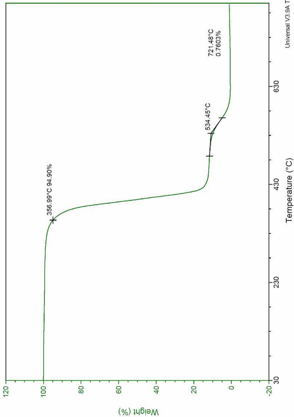
Figure. 3-85 TGA Thermogram of Epoxy III/CA I /CA III=1/0.1/0.9
