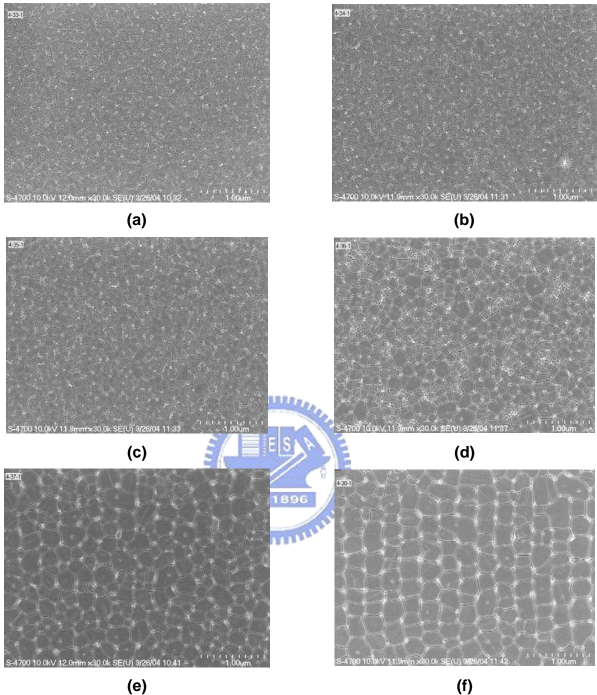
Fig. 2-26 SEM micrographs of excimer laser crystallized poly-Silicon films after Secco etching for 60sec treatment. The applied laser energy densities are (a) 330, (b) 340, (c) 350, (d) 360 (e) 370 (f) 380 \text{mJ}/\text{cm}^2 . The laser energy 950mJ, frequency 300Hz, power 285W, scan speed 6mm/sec, pitch 0.02mm, beam width 0.4mm, pre treatment clean with O3 20ppm for 500sec
