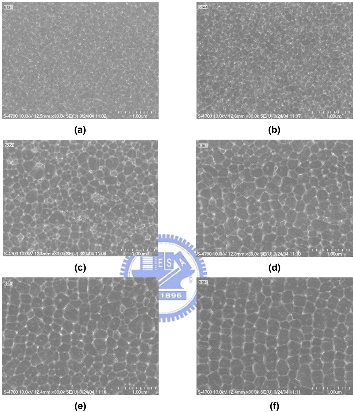
Fig. 2-38 SEM micrographs of excimer laser crystallized poly-Silicon films after Secco etching for 60sec treatment. The applied laser energy densities are (a) 330, (b) 340, (c) 350, (d) 360 (e) 370 (f) 380 \text{mJ}/\text{cm}^2 . The laser energy 950mJ, frequency 300Hz, power 285W, scan speed 6mm/sec, pitch 0.02mm, beam width 0.4mm, pre treatment clean with H 2 O 2 30% for 540sec
