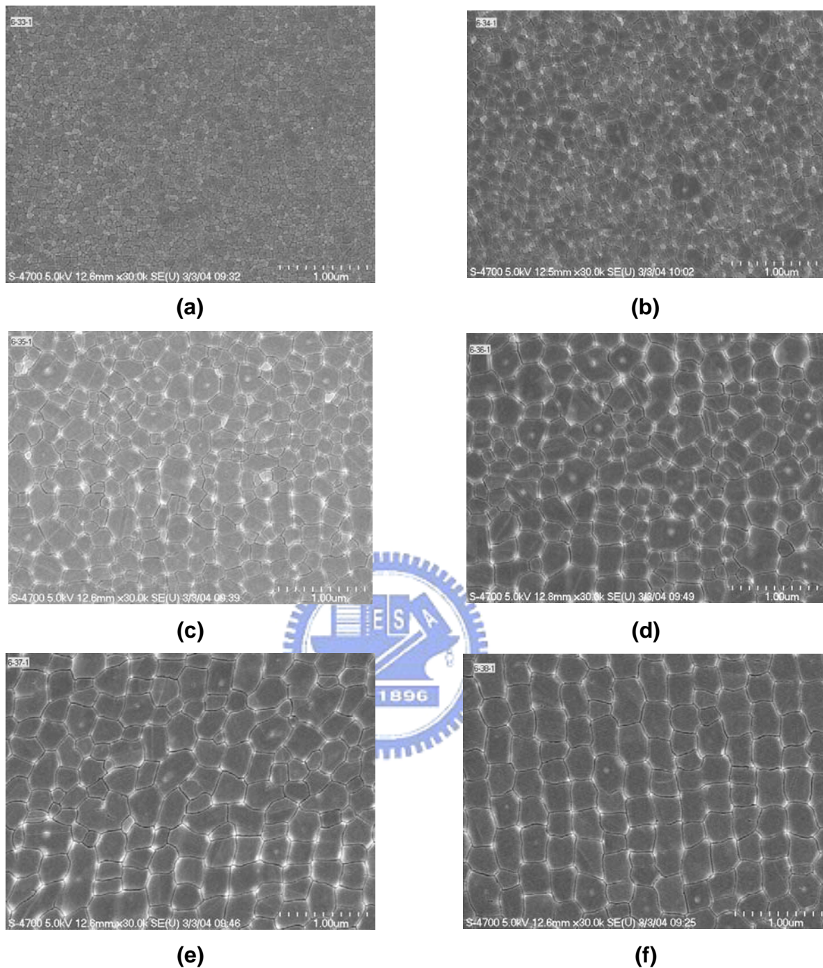
Fig. 2-44 SEM micrographs of excimer laser crystallized poly-Silicon films after Secco etching for 60sec treatment. The applied laser energy densities are (a) 330, (b) 340, (c) 350, (d) 360 (e) 370 (f) 380 \text{mJ}/\text{cm}^2 . The laser energy 950mJ, frequency 300Hz, power 285W, scan speed 6mm/sec, pitch 0.02mm, beam width 0.4mm, pre treatment clean with UV exposure \lambda 254\text{nm} for 400sec
