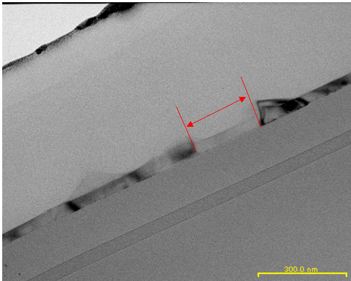
Fig. 2-51 Cross-section TEM micrographs of the crystallized by excimer laser irradiation poly silicon thin film
