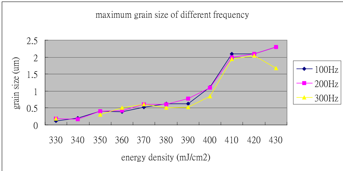
Fig. 3-3 The maximum grain size distribution of different laser frequency with pre treatment clean of HF+O 3 after excimer laser irradiation with different laser energy density at room temperature.
