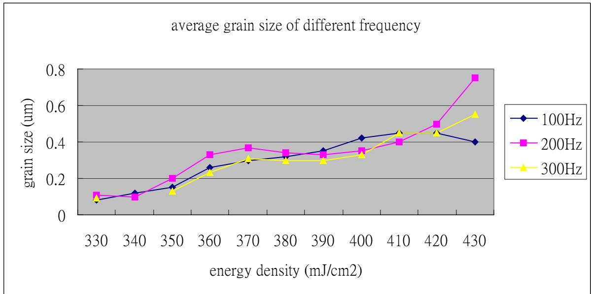
Fig. 3-1 The average grain size distribution of different laser frequency with pre treatment clean of HF+O 3 after excimer laser irradiation with different laser energy density at room temperature.
