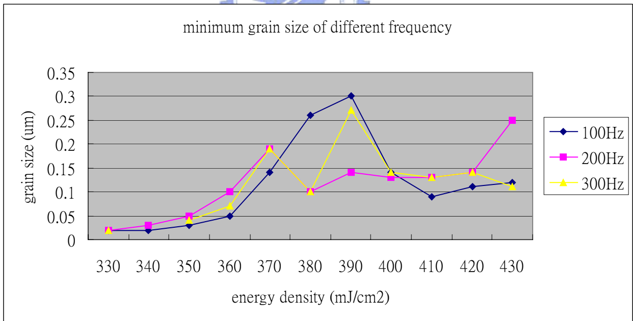
Fig. 3-2 The minimum grain size distribution of different laser frequency with pre treatment clean of HF+O 3 after excimer laser irradiation with different laser energy density at room temperature.
