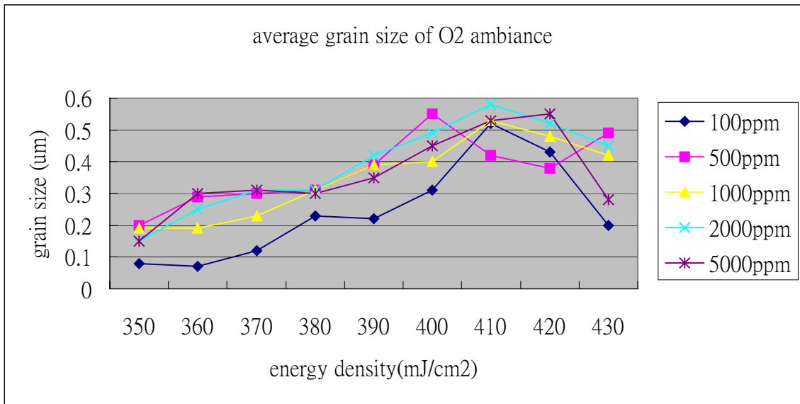
Fig. 3-19 The average grain size distribution of different irradiation ambience with pre treatment clean of HF1% for 30sec after excimer laser irradiation with different laser energy density at room temperature.
