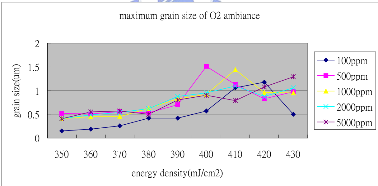
Fig. 3-20 The maximum grain size distribution of different irradiation ambience with pre treatment clean of HF1% for 30sec after excimer laser irradiation with different laser energy density at room temperature.
