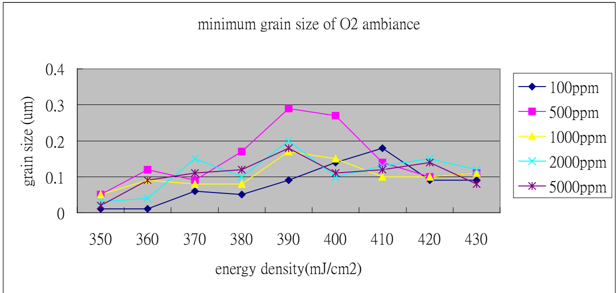
Fig. 3-21 The minimum grain size distribution of different irradiation ambience with pre treatment clean of HF1% for 30sec after excimer laser irradiation with different laser energy density at room temperature.
