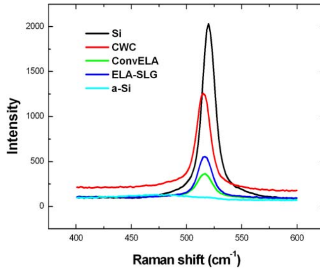
Fig. 4-1 The Raman spectrum of silicon and poly-silicon films
