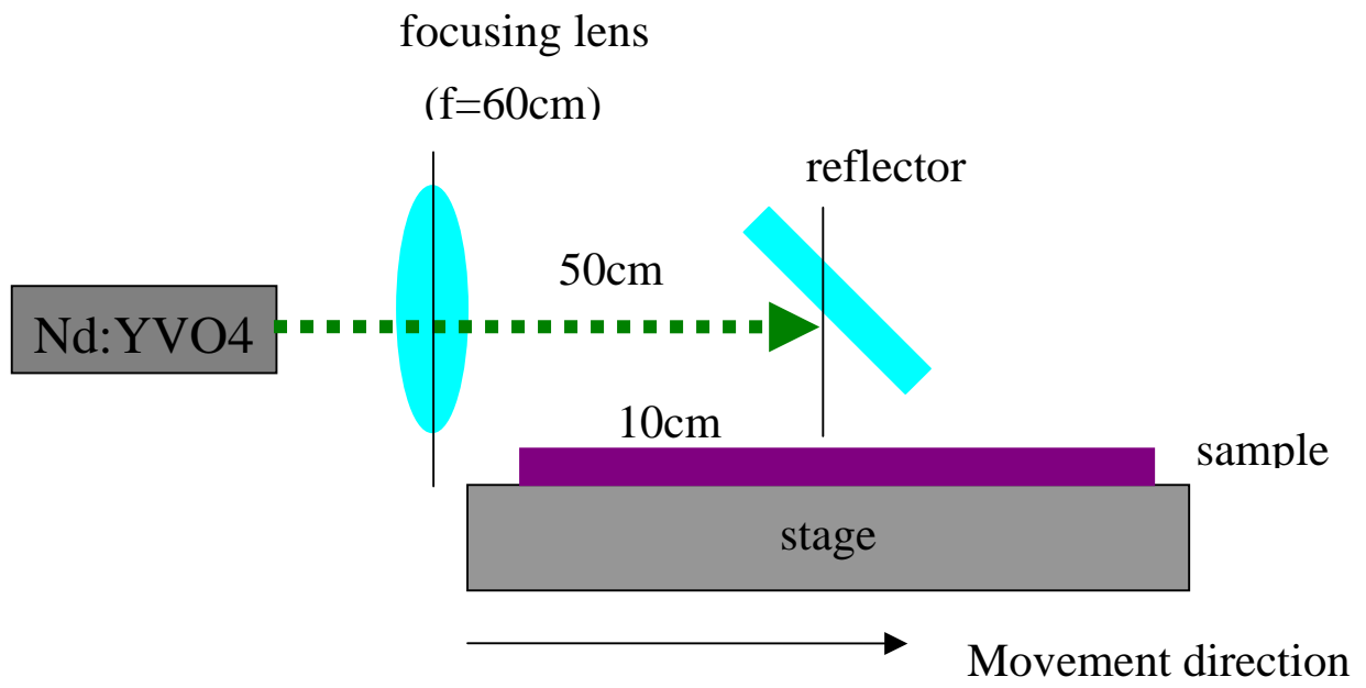
Fig. 4-3 A brief schematic of the continuing wave laser system.
