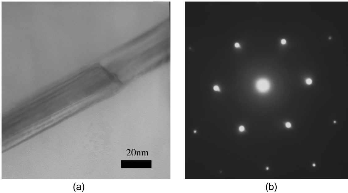
Fig. 4-26 High-magnification cross-sectional TEM image (a) and electron diffraction pattern (b) of a CW crystallite. The diffraction pattern reveals that the crystallite exhibits \langle 111 \rangle orientation along the direction of film grain growth.
