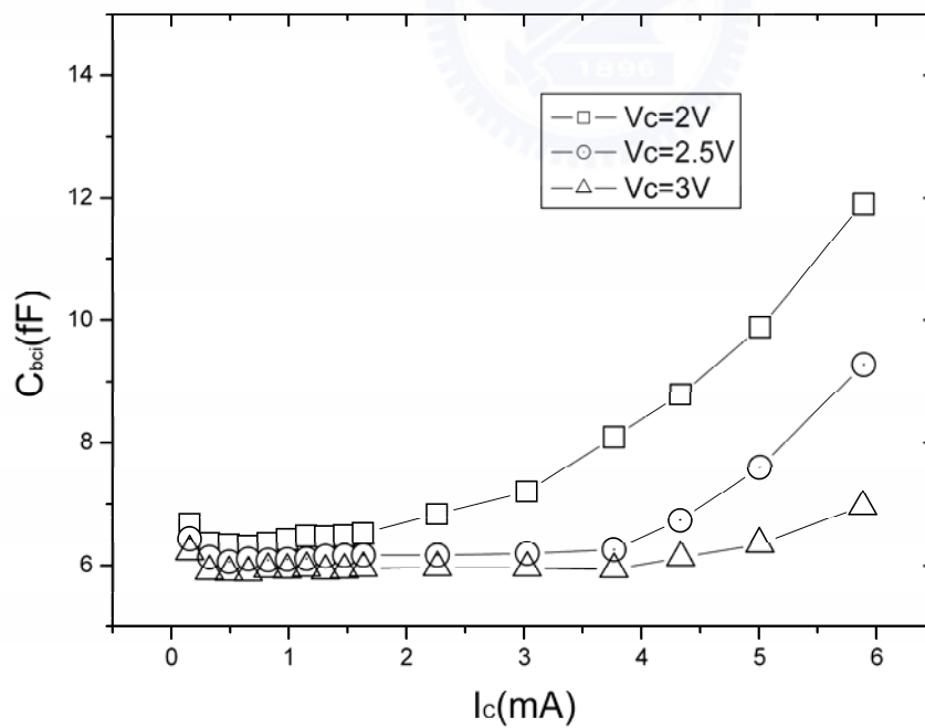
Fig. 3-5 Intrinsic base-collector capacitance versus collector current.
