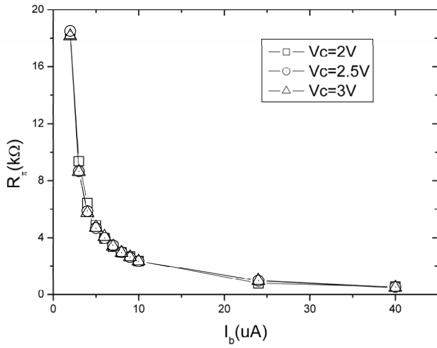
Fig. 3-3 Base-emitter resistance versus base current.
