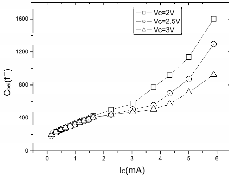
Fig. 3-4 Intrinsic base-emitter capacitance versus collector current.
