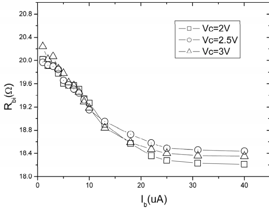
Fig. 3-6 Intrinsic base resistance versus base current.
