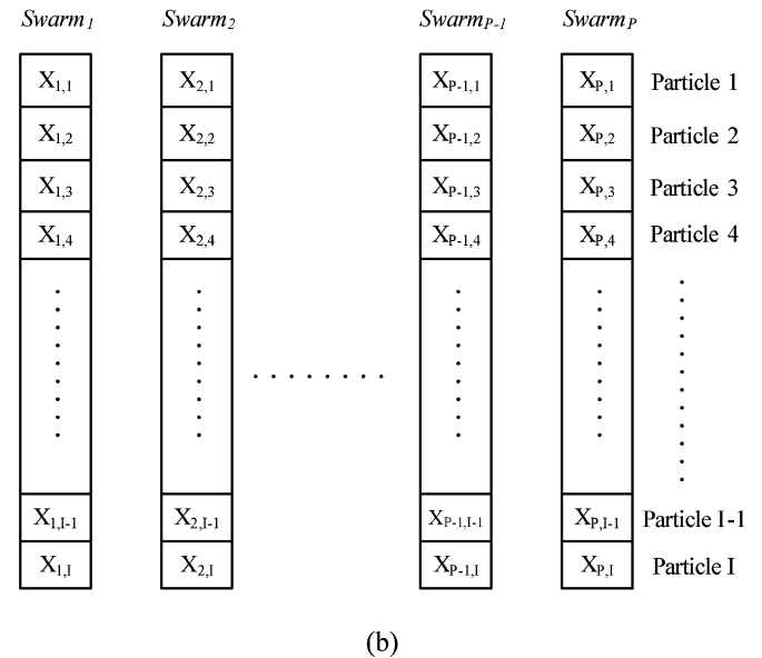
Fig. 5. Framework of (a) PSO and (b) CPSO.
