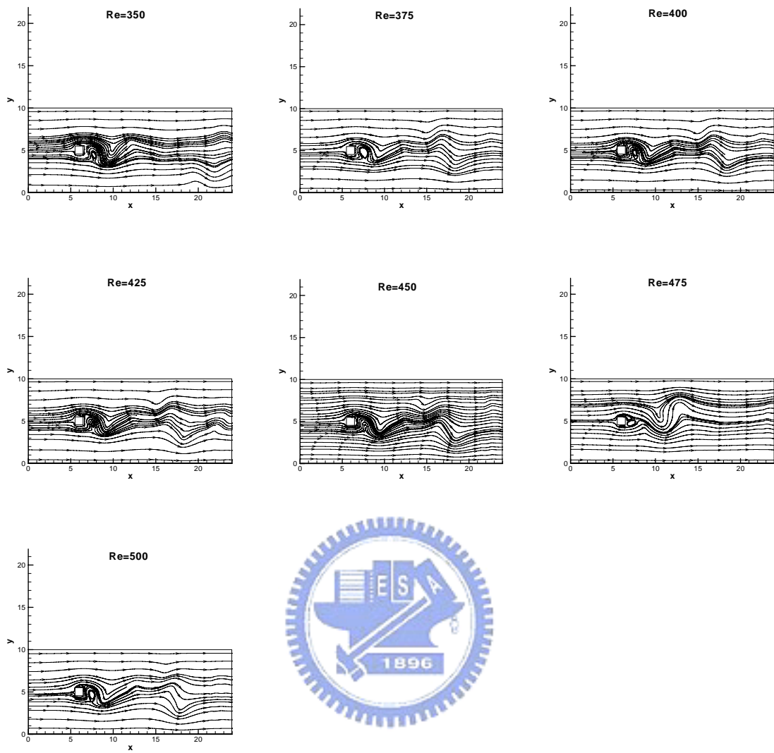
Figure 6-17. Variation of instantaneous streamlines with Reynolds number (Uniform free stream).
