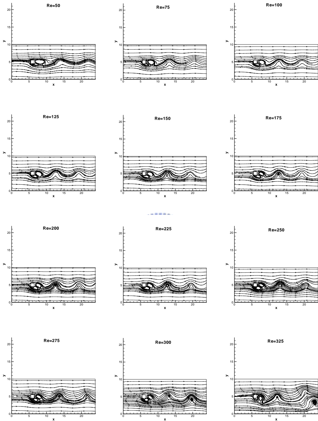
Figure 6-18. Variation of instantaneous streamlines with Reynolds number (Velocity ratio 3:1 and L1=6 ). Continue...
