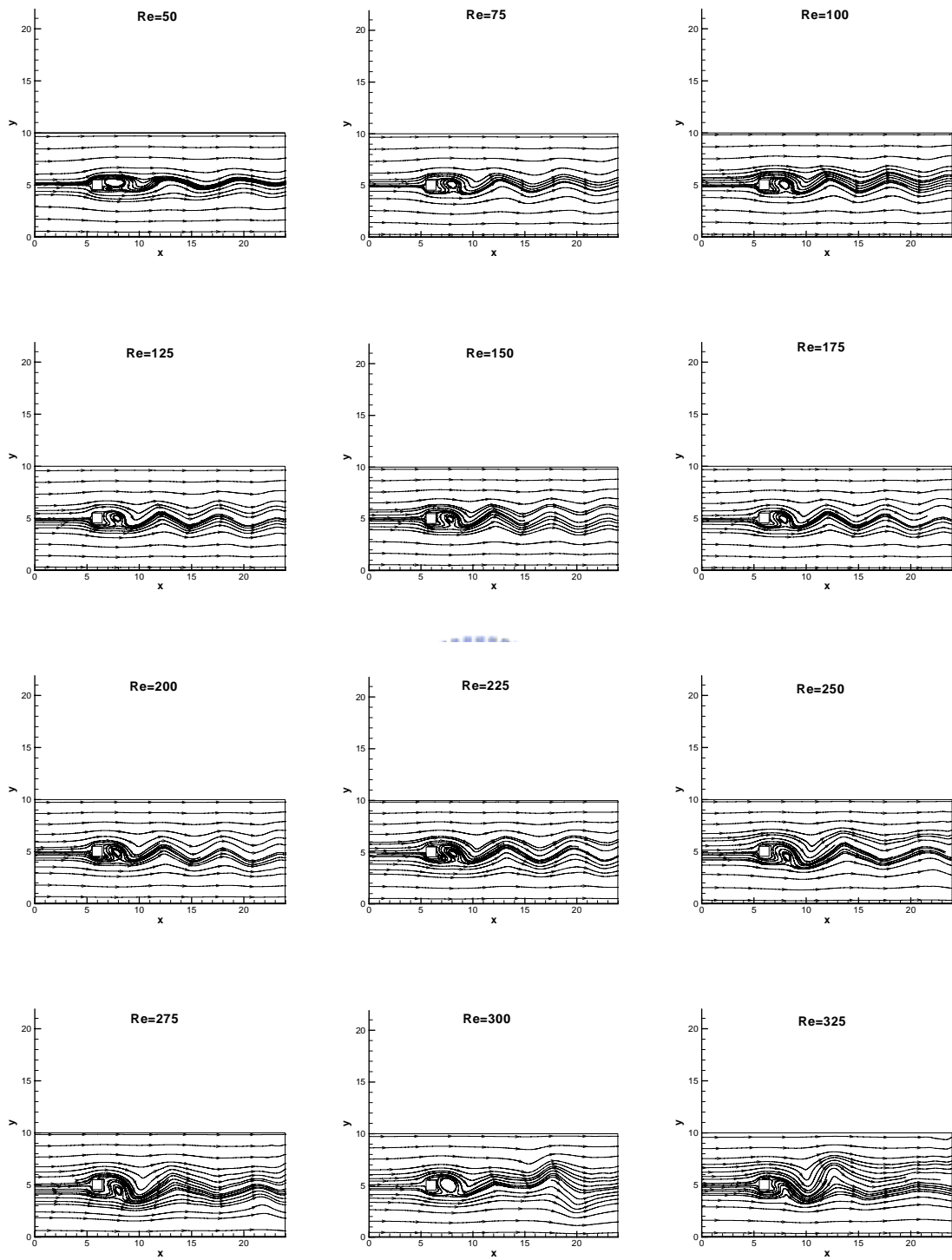
Figure 6-17. Variation of instantaneous streamlines with Reynolds number (Uniform free stream). Continue...
