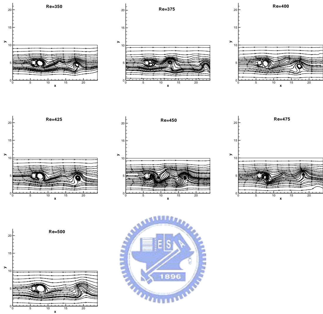
Figure 6-19. Variation of instantaneous streamlines with Reynolds number (Velocity ratio 3:2 and L1=6 ).
