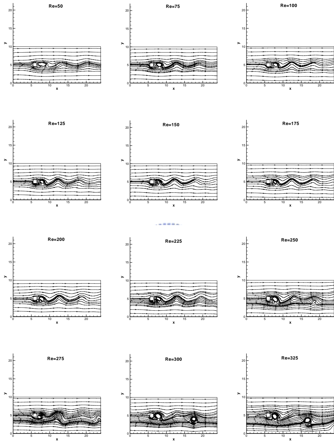
Figure 6-19. Variation of instantaneous streamlines with Reynolds number (Velocity ratio 3:2 and L1=6 ). Continue...
