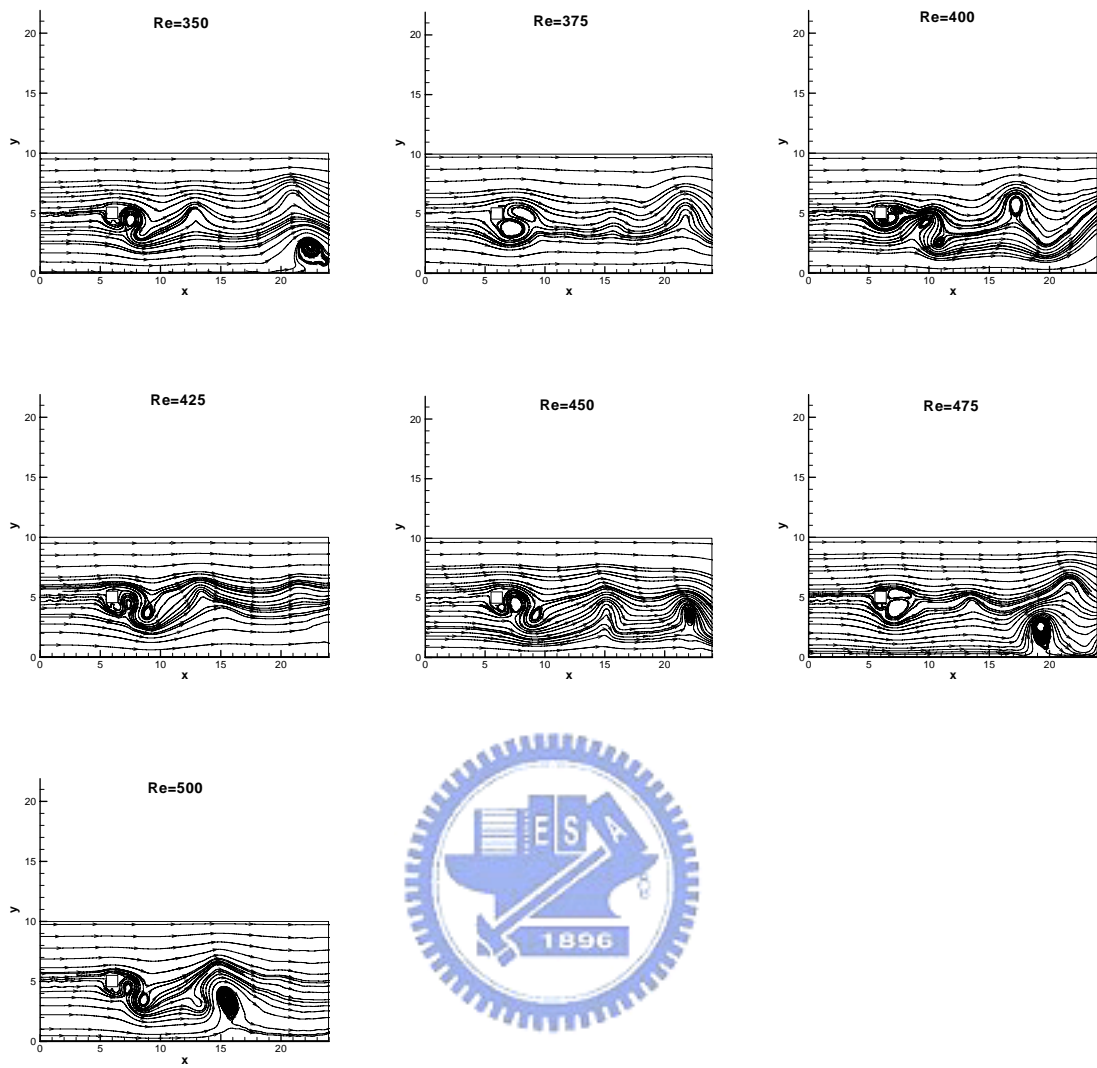
Figure 6-18. Variation of instantaneous streamlines with Reynolds number (Velocity ratio 3:1 and L1=6 ).
