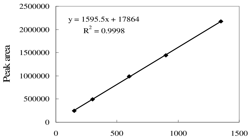
2,5-dimethoxybenzaldehyde conc(mg/L)
