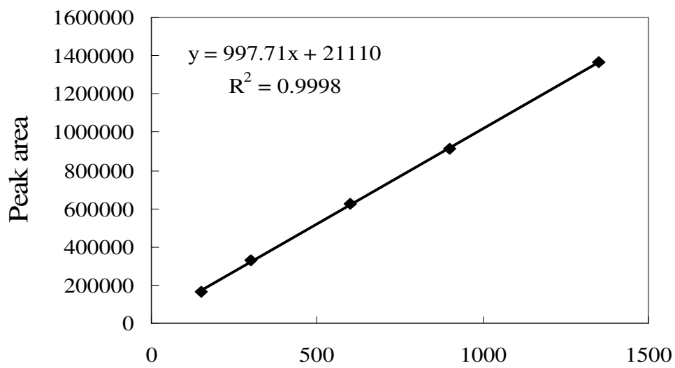
4-chlorobenzaldehyde conc(mg/L)
