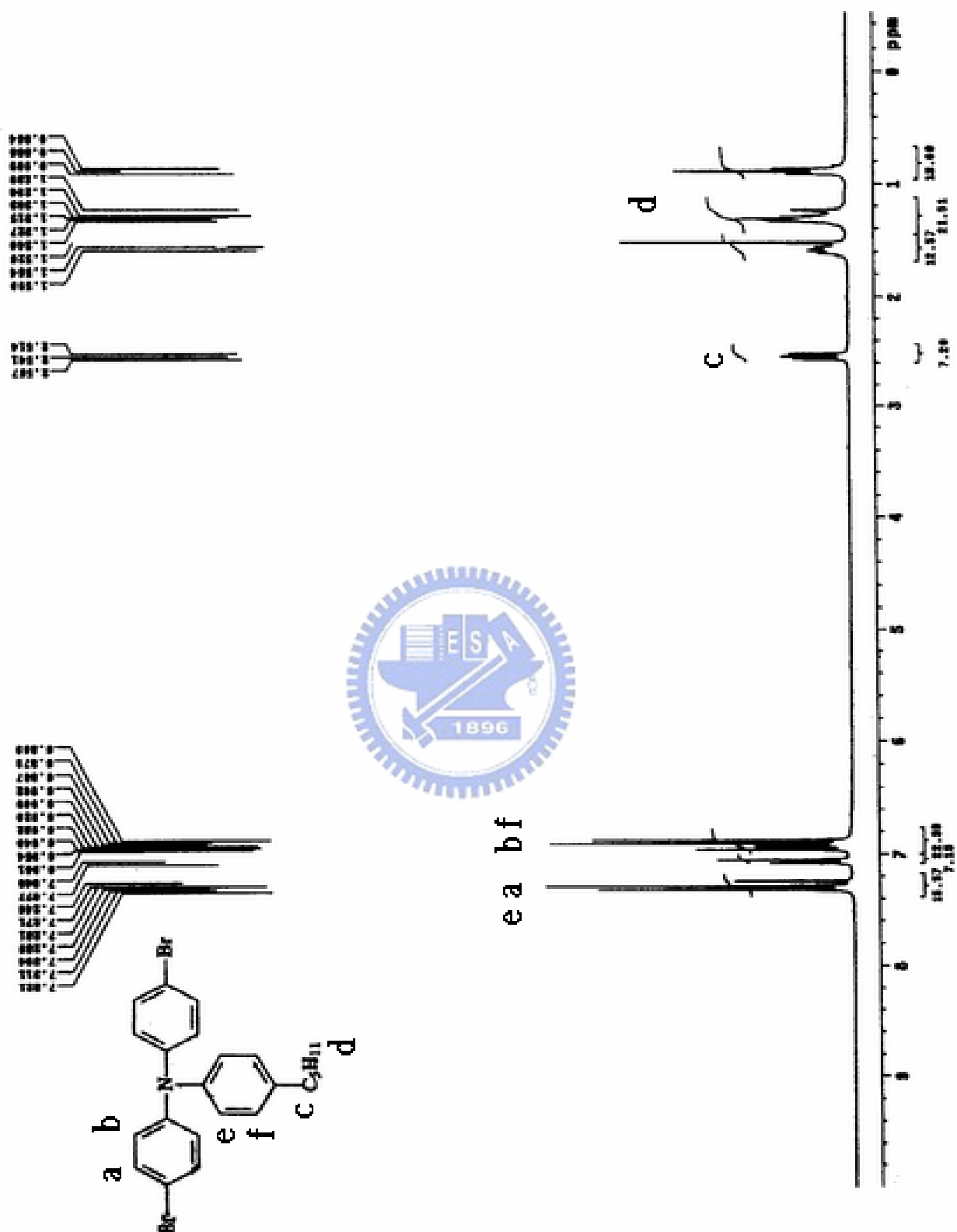
附圖 5. 1 H-NMR spectrum of M5
