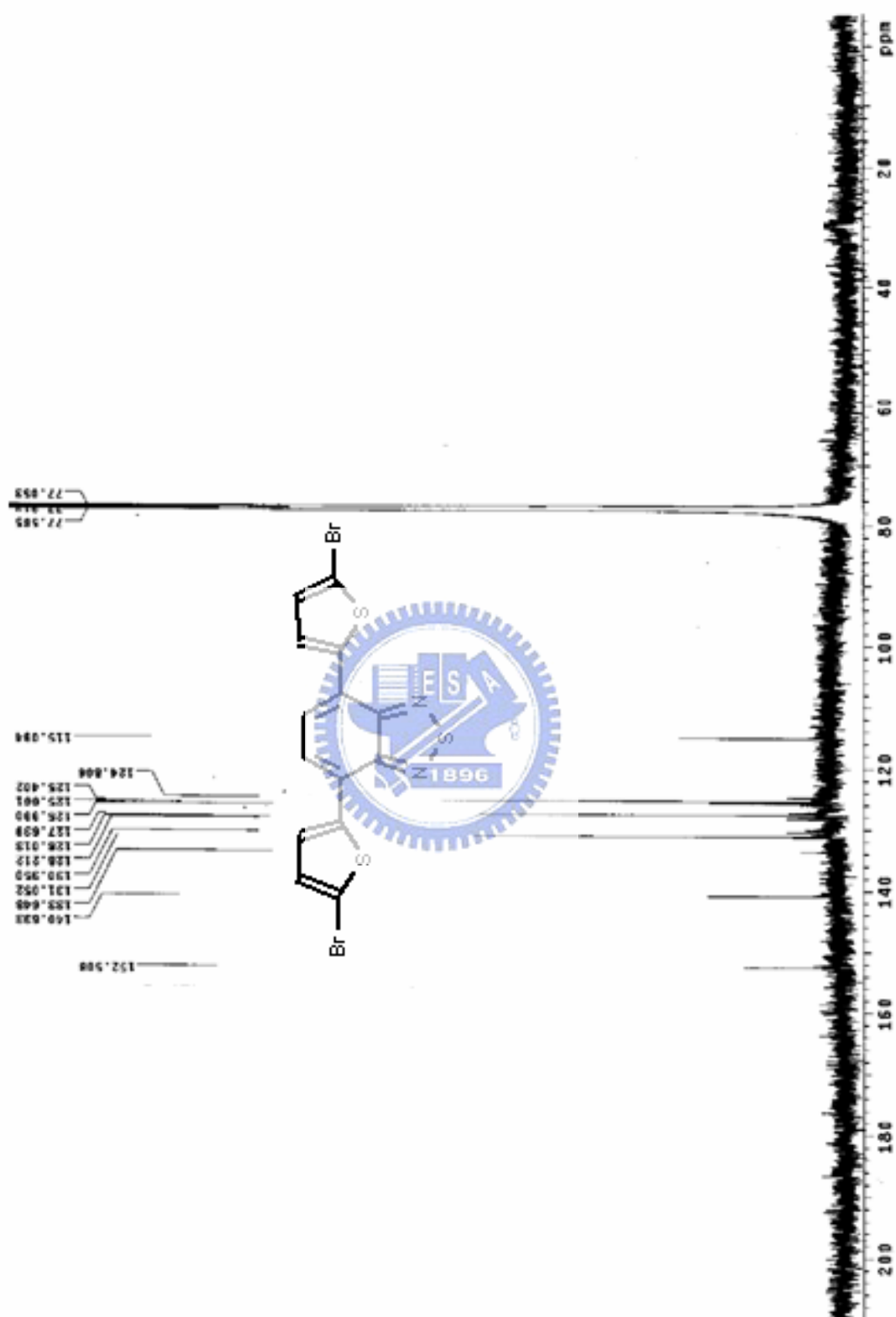
附圖 14. ^{13}\text{C} -NMR spectrum of M7
