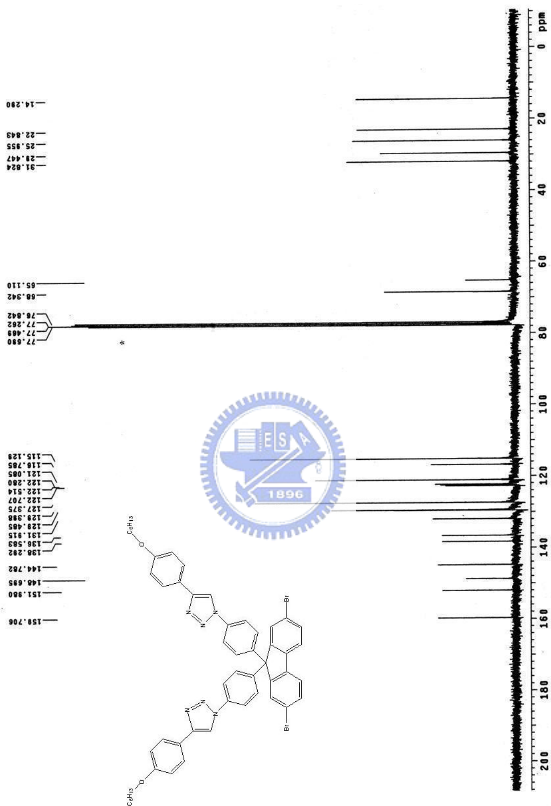
附圖 9. ^{13}\text{C} -NMR spectrum of M2
