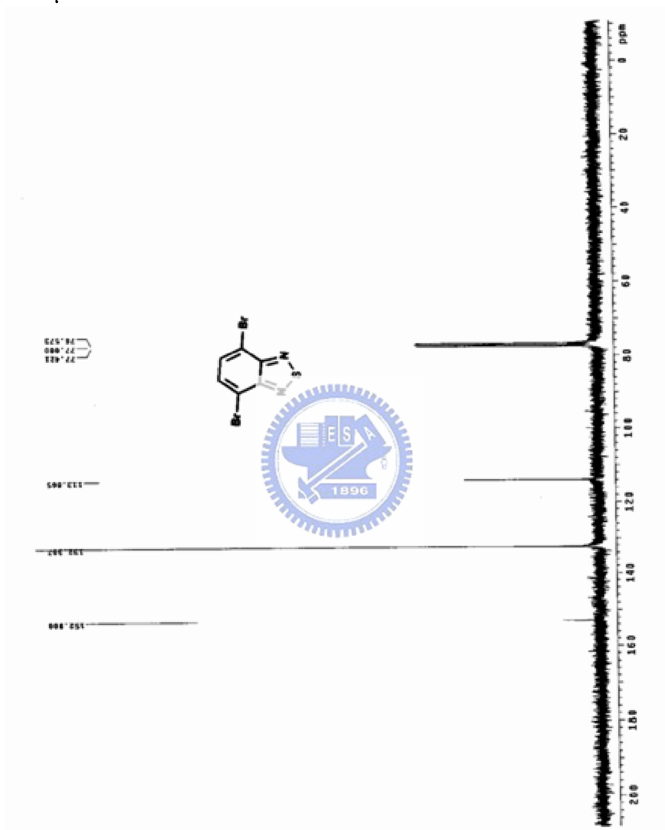
附圖 13. ^{13}\text{C} -NMR spectrum of M6
