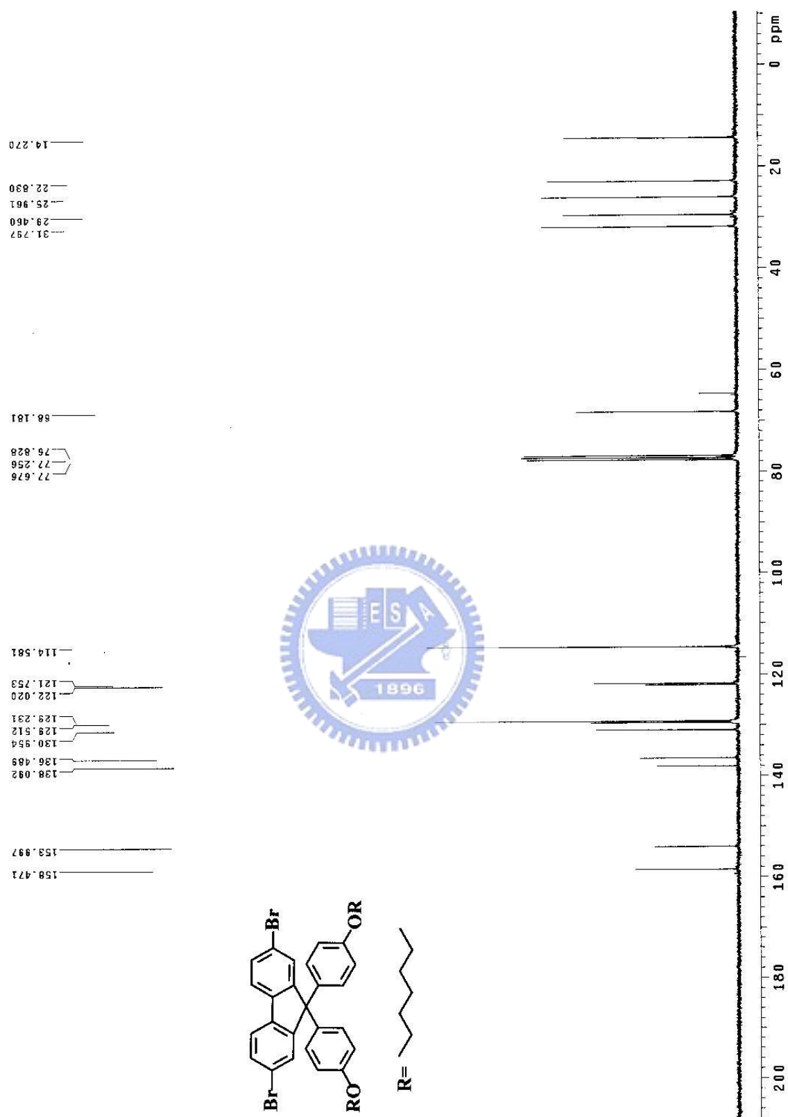
附圖 10. ^{13}\text{C} -NMR spectrum of M3
