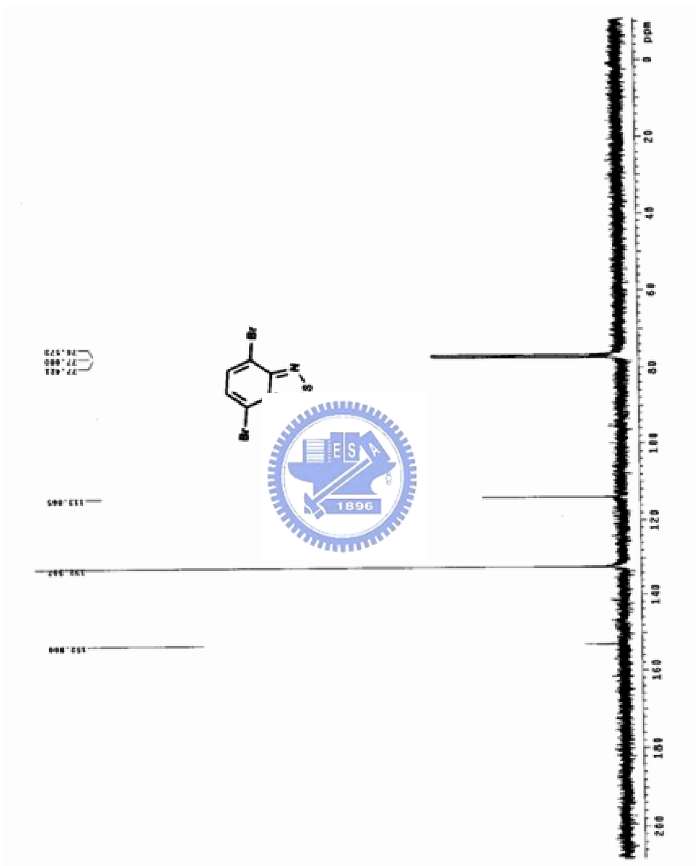
附圖. 19 ^{13}\text{C} -NMR spectrum of M6
