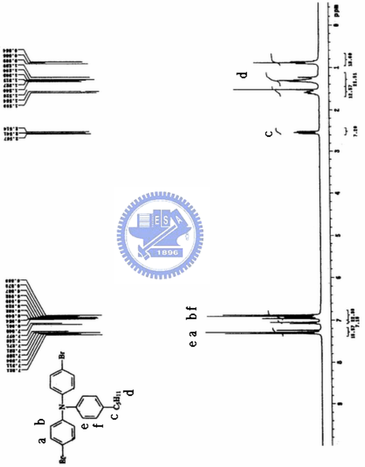
附圖.4 ^1\text{H-NMR} spectrum of M4
