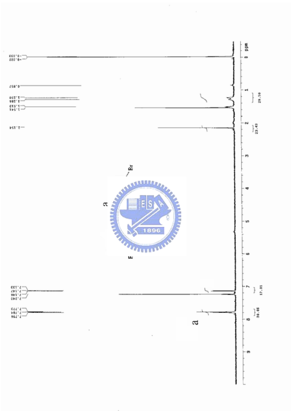
附圖. 10 ^1\text{H-NMR} spectrum of M7
