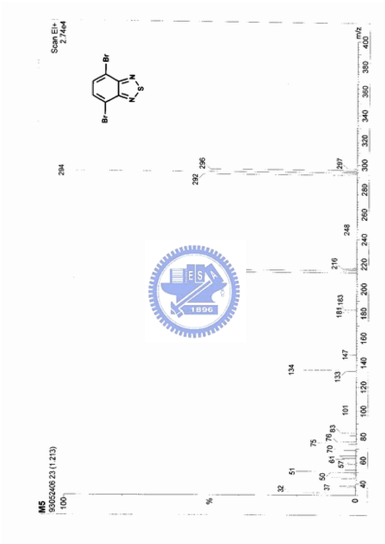
附圖. 29 Mass spectrum of M6
