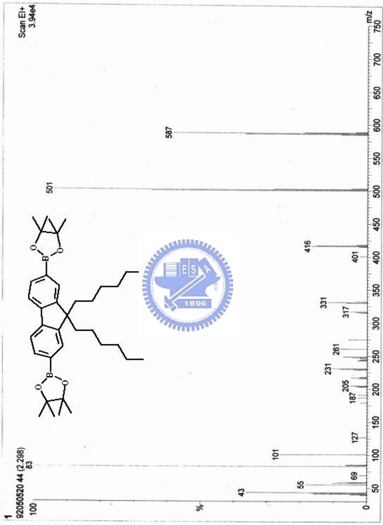
附圖. 25 Mass spectrum of M2
