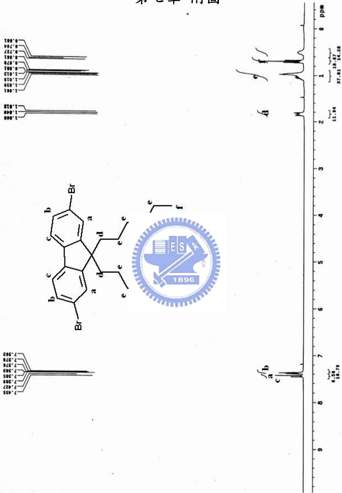
附圖. 1 ^1\text{H-NMR} spectrum of M1
