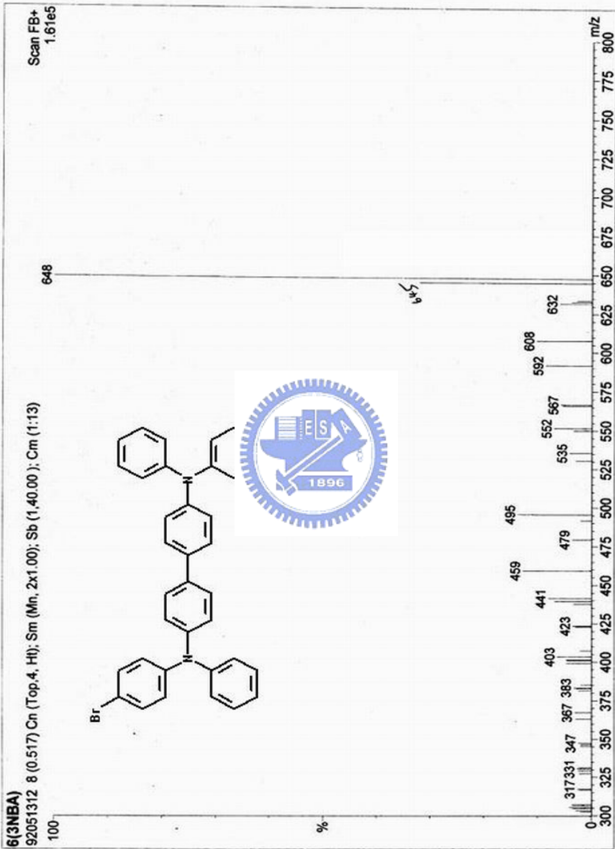
附圖. 28 Mass spectrum of M5
