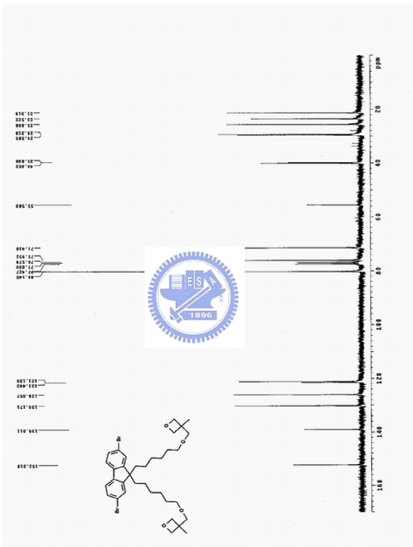
附圖. 16 ^{13}\text{C} -NMR spectrum of M3
