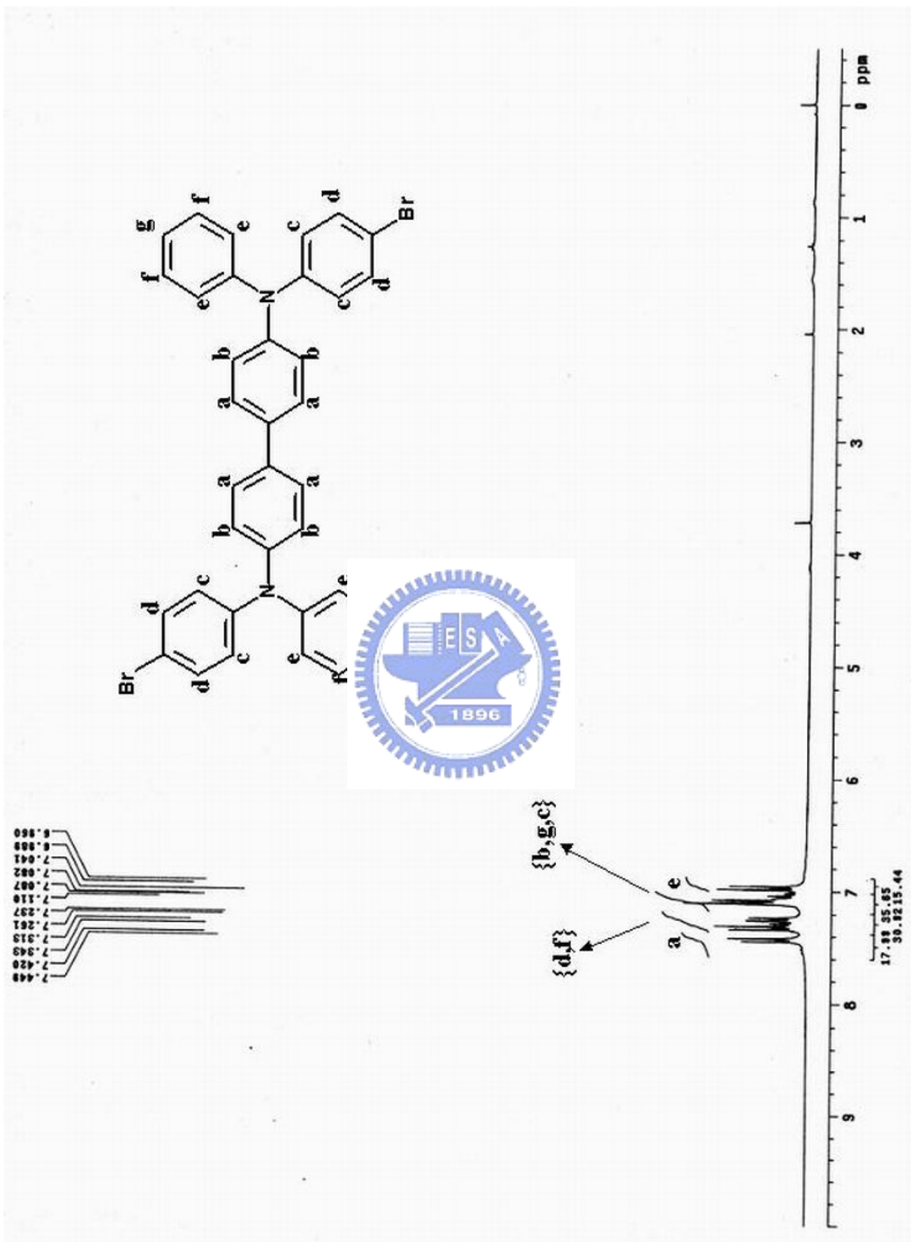
附圖. 5 ^1\text{H-NMR} spectrum of M5
