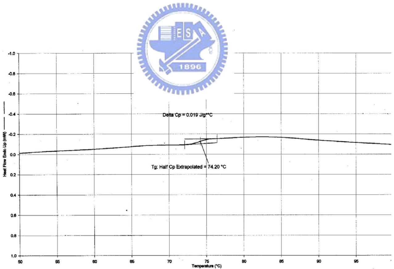
附圖 9. DSC thermogram of P1
