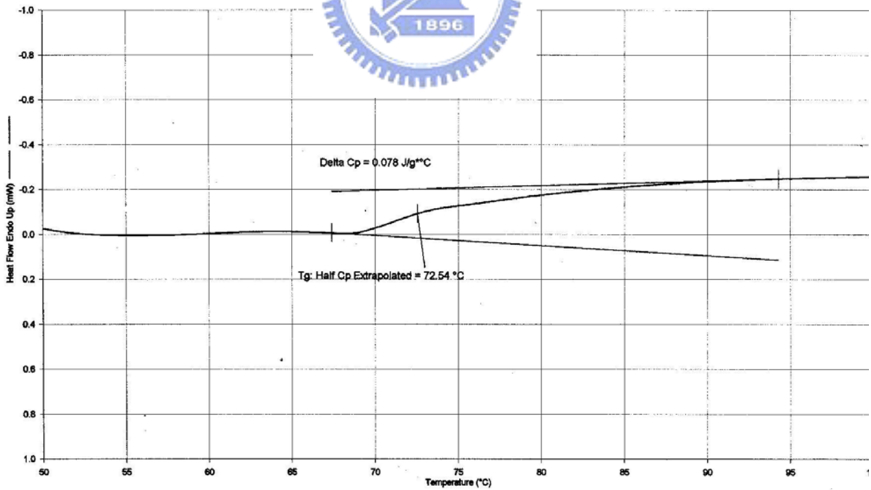
附圖 13. DSC thermogram of P3
