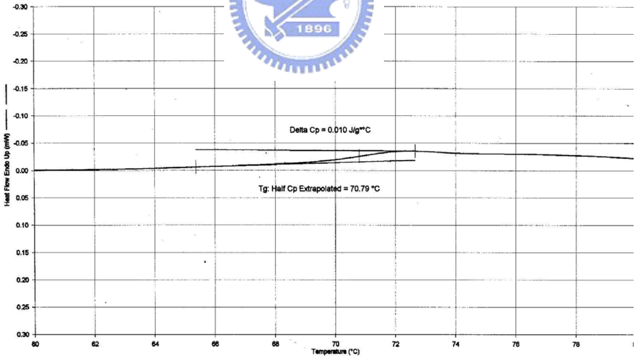
附圖 16. DSC thermogram of P4
