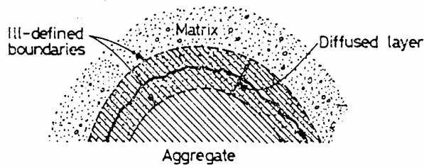
圖 2-1 Diagrammatic representation of interactions at the aggregate-matrix interface [3, 4]
