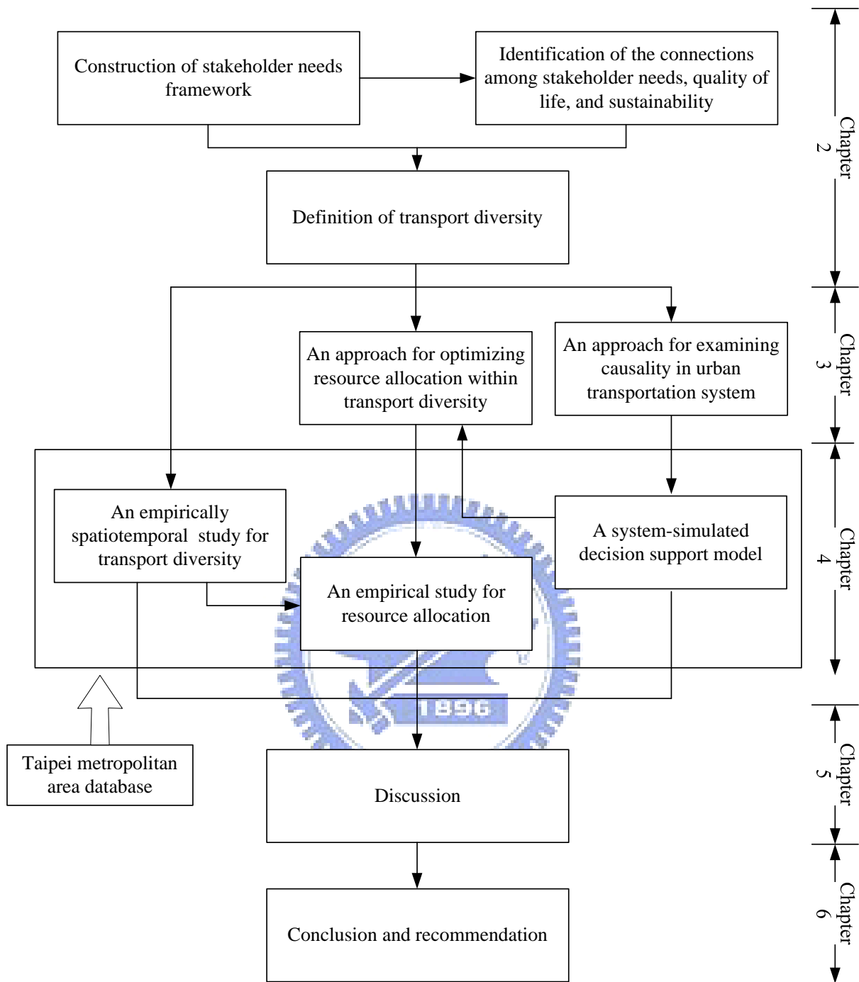
FIGURE 1-1 Research framework
