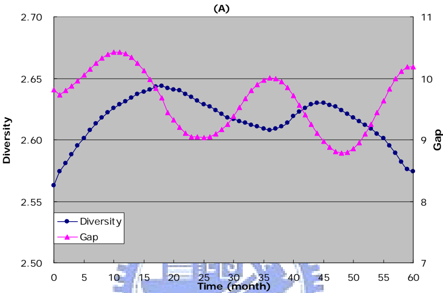
FIGURE 4-5 Diversity and gap in baseline simulation
