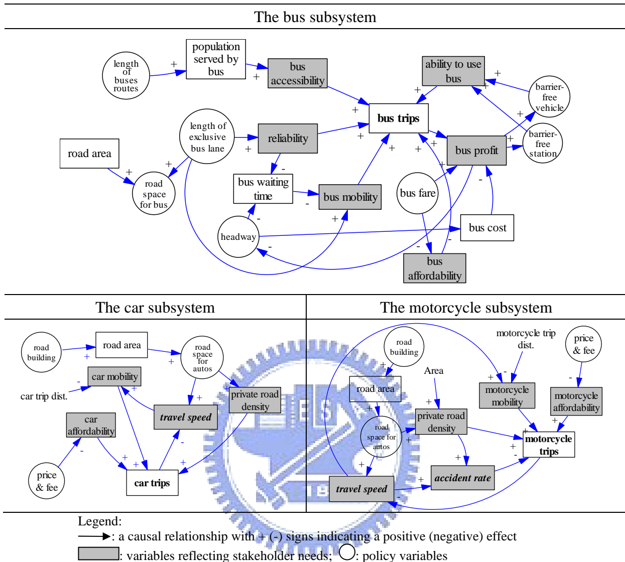
FIGURE 3-4 Feedback structures in subsystems
