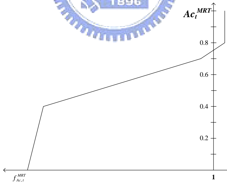
FIGURE 3-5 Function of adjustment factor of MRT accessibility
