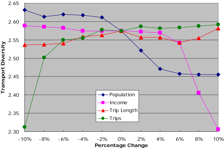
FIGURE 4-3 Sensitivity analysis for proposed simulation model
