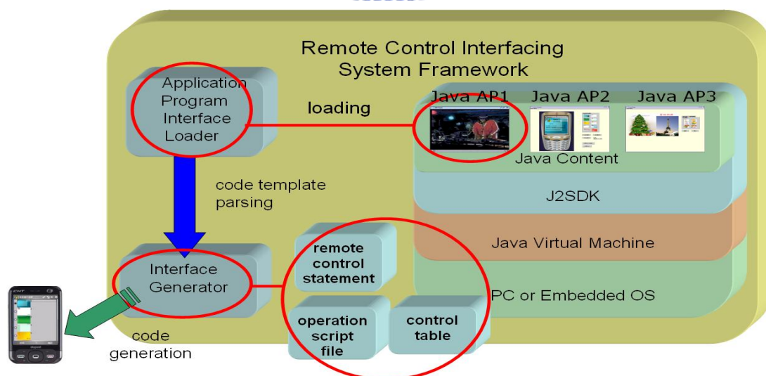
圖 20、Remote Control Interfacing System Framework
