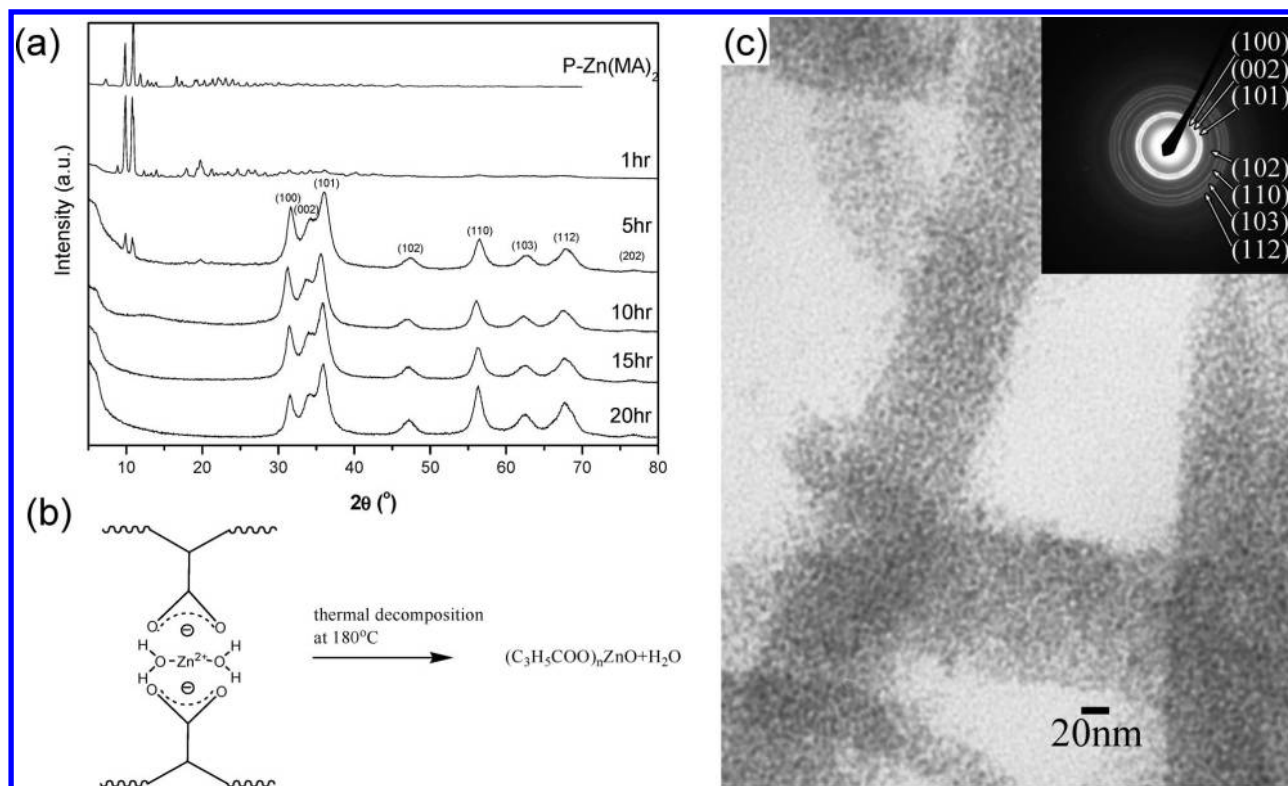
Figure 7. (a) XRD diffraction patterns of \text{P-Zn}(\text{MA})_2 nanofibers oxidized at 180^\circ\text{C} for various periods of time; (b) the thermal decomposition mechanism of \text{ZnO} nanoparticle formation; (c) TEM image of the \text{P-ZnO}(\text{MA})_2 nanofiber composite obtained after oxidation at 180^\circ\text{C} for 15 h.
