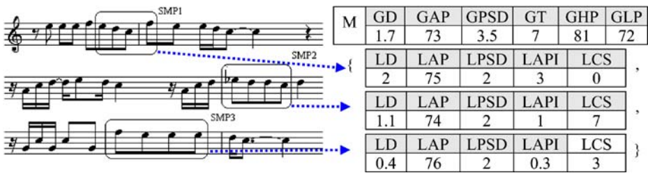
Fig. 2 An example of a music object with three significant segments and its feature representation (excerpt from the song “Don’t let the sun go down on me.”)
