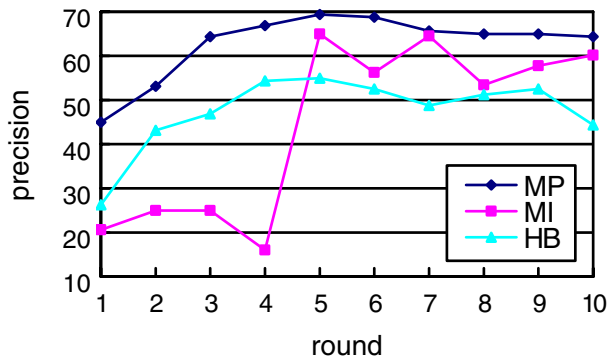
Fig. 4 Performance comparisons of three feedback strategies
