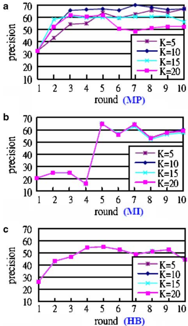
Fig. 5 Performances with different K as a function of the round number for different system feedback strategies, a the most positive, b the most informative, c the hybrid
