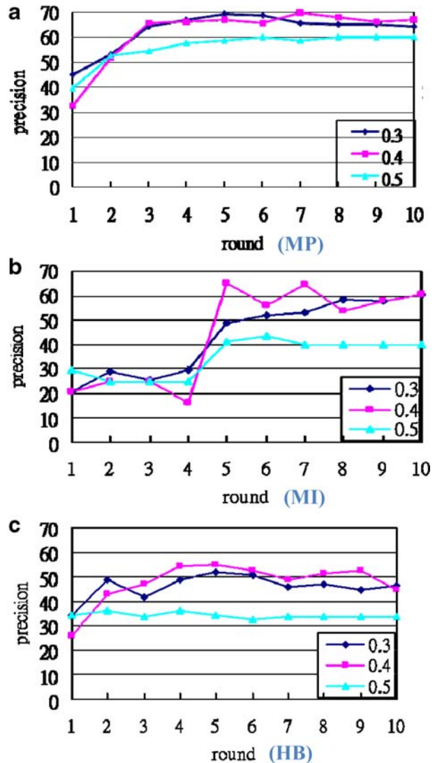
Fig. 6 Performances with different significance selection thresholds as a function of the round numbers for different system feedback strategies, a the most positive, b the most informative c the hybrid
