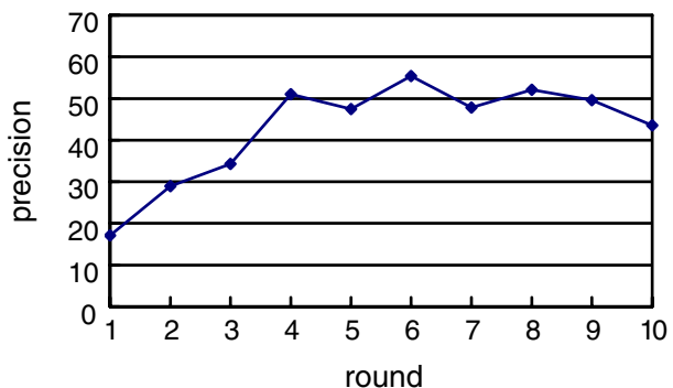
Fig. 7 Performances as a function of the round numbers for Most-Positive feedback strategies on music genre database
