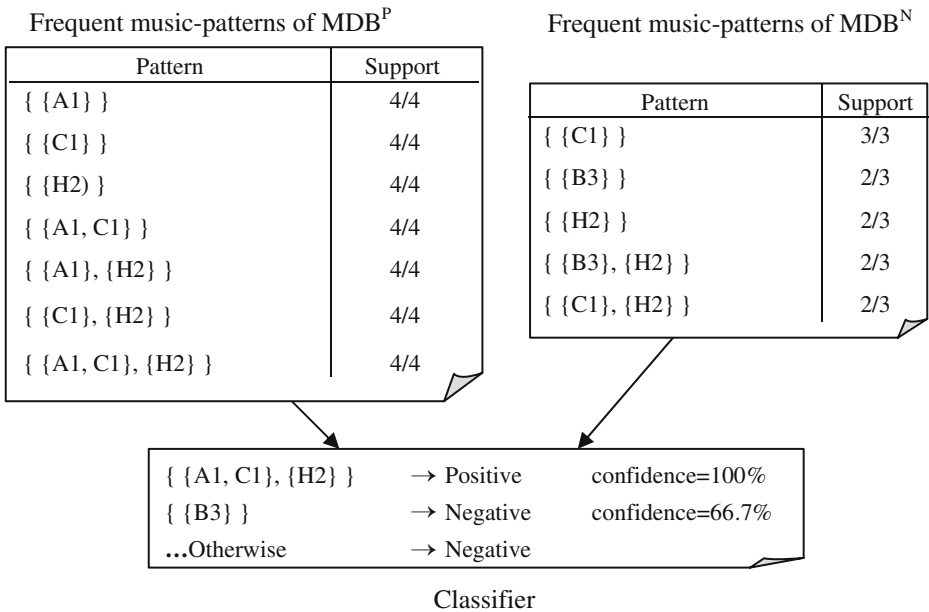
Fig. 3 An example of a classifier learned from Tables 4 and 5
