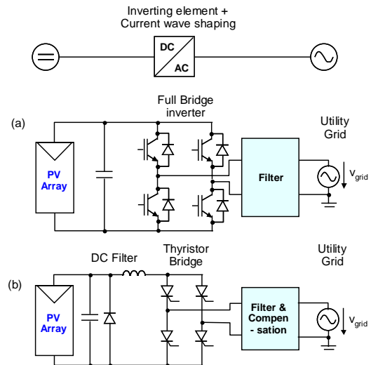
Fig. 8. Transformerless PV Inverters.
