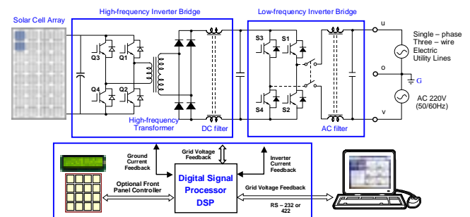
Fig. 9. A Two-stage high-frequency transformer PV Inverter.
