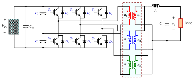
Fig. 13. Multiphase half-bridge inverter topology.
