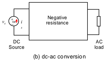
Fig. 3. Characteristics of ac-dc and dc-ac power conversion.
