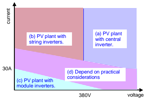
Fig. 3. Classification of grid-connected PV inverter systems according to power ratings.
