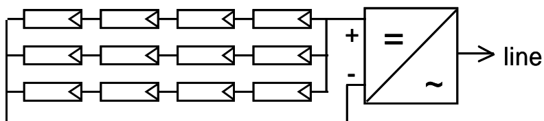
(a) PV plant with central inverter.
