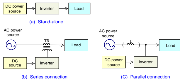
Fig. 1. Classification of inverters.
