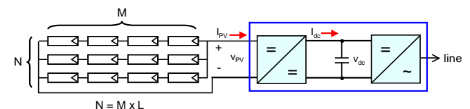
Fig. 10. Configuration of PV modules in a PV Inverter system.
