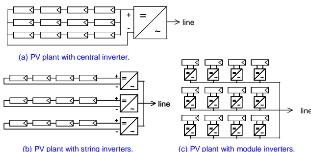
Fig. 2 Configurations of grid-connected PV inverter systems.
