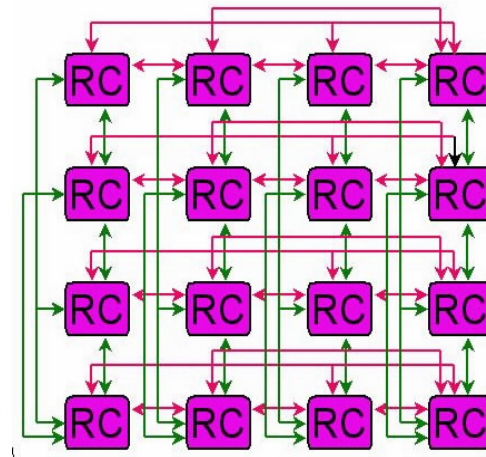
Figure 4. Reconfigurable Cell
