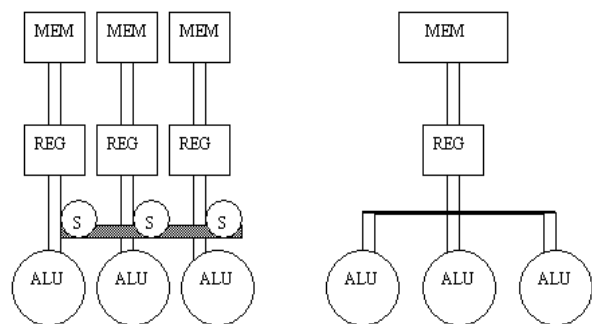
Figure 1. RAW vs Superscalar
