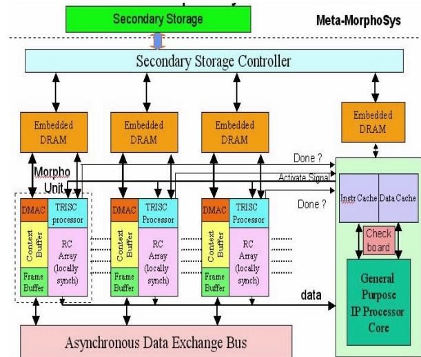
Figure 6. meta-MorphoSys Architecture
