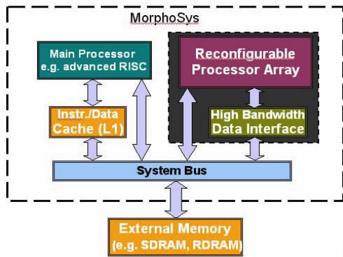
Figure 3. MorphoSys Architecture
