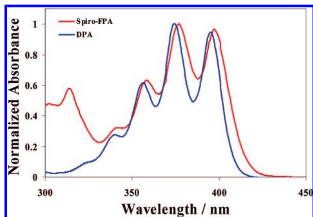
Figure 4. Absorbance spectra of solutions of 52 \mu\text{M} spiro-FPA and 56 \mu\text{M} DPA in 3:1 PhH/MeCN.
