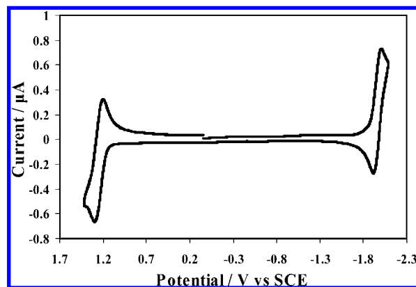
Figure 2. Cyclic voltammogram of 0.5 mM spiro-FPA in 3:1 benzene/acetonitrile. Scan rate = 200 mV/s.
