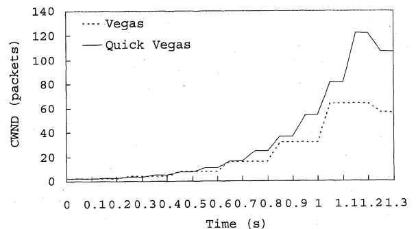
Fig. 2 Congestion window evolutions of Vegas and Quick Vegas during slow-start phase.
