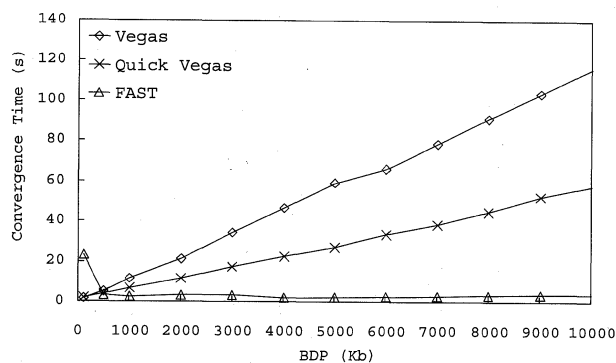
Fig. 10 Convergence time of new connections.
