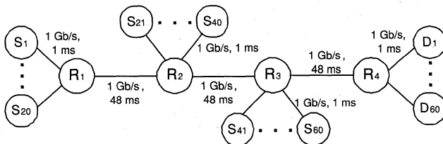
Fig. 15 Network configuration for the connections with different RTTs .
