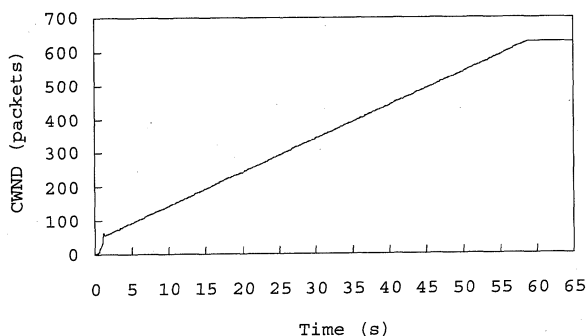
Fig. 1 Congestion window evolution of a Vegas connection.
