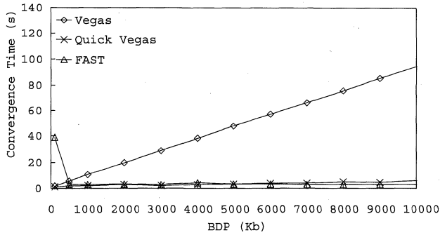
Fig. 11 Convergence time of connections when available bandwidth is halved.
