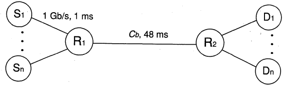
Fig. 6 Network configuration for the connections with the same RTT .
