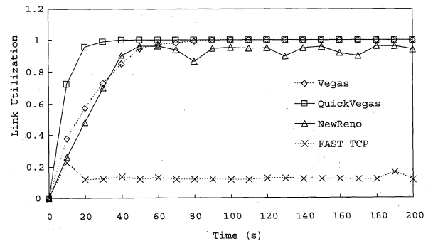
Fig. 16 Bottleneck link utilization for the connections with different RTTs .
