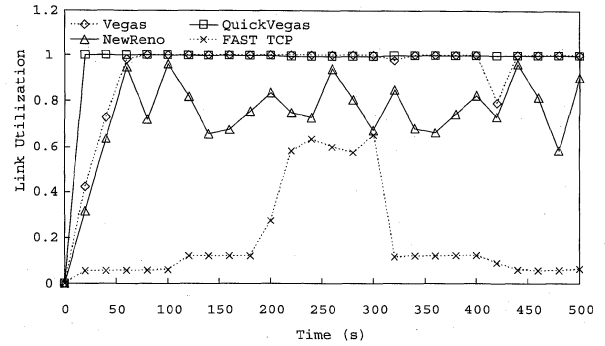
Fig. 13 Bottleneck Link Utilization for the connections with the same RTT.
