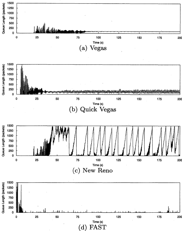
Fig. 17 Queue status of the bottleneck for the connections with different RTTs .
