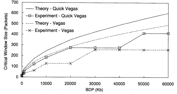
Fig. 4 Critical window sizes for Vegas and Quick Vegas in different BDPs.
