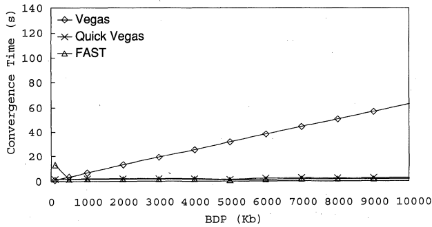
Fig. 12 Convergence time of connections when available bandwidth is doubled.
