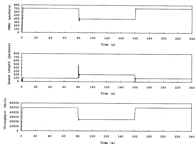
Fig. 9 Basic behavior of FAST.
