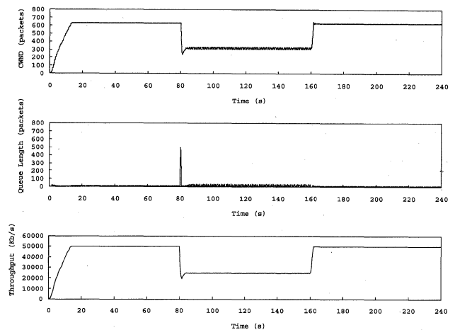
Fig. 8 Basic behavior of Quick Vegas.
