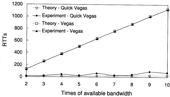
Fig. 5 The number of RTT s needed for Vegas and Quick Vegas reaches new equilibrium states.
