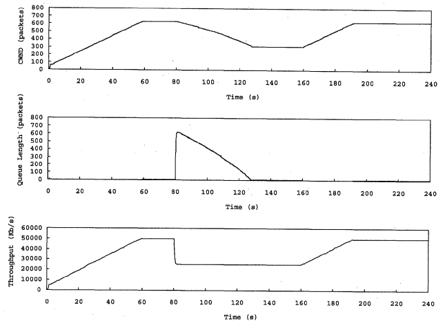
Fig. 7 Basic behavior of Vegas.
