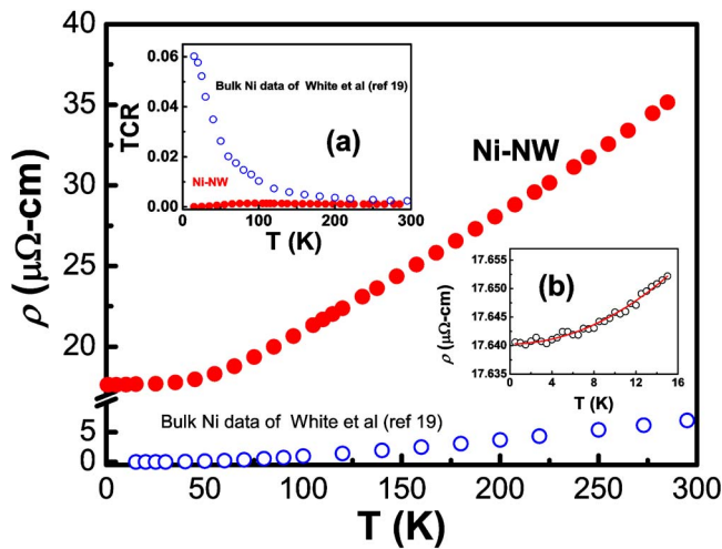
FIG. 2. (Color online) The resistivity \rho(T) of the Ni-NW (solid circles) and the bulk (open circles) from White et al. Inset (a): the temperature dependence of TCR of the Ni-NW (solid circles) and the bulk (open circles) from White et al. Inset (b): the temperature dependence of resistivity of Ni-NW and the curve fit of \rho = \rho_0 + aT^n , with \rho_0 = 17.6 \mu\Omega \text{ cm} , a = 5 \times 10^{-5} \mu\Omega \text{ cm/K}^2 , and the power n \sim 2 .
