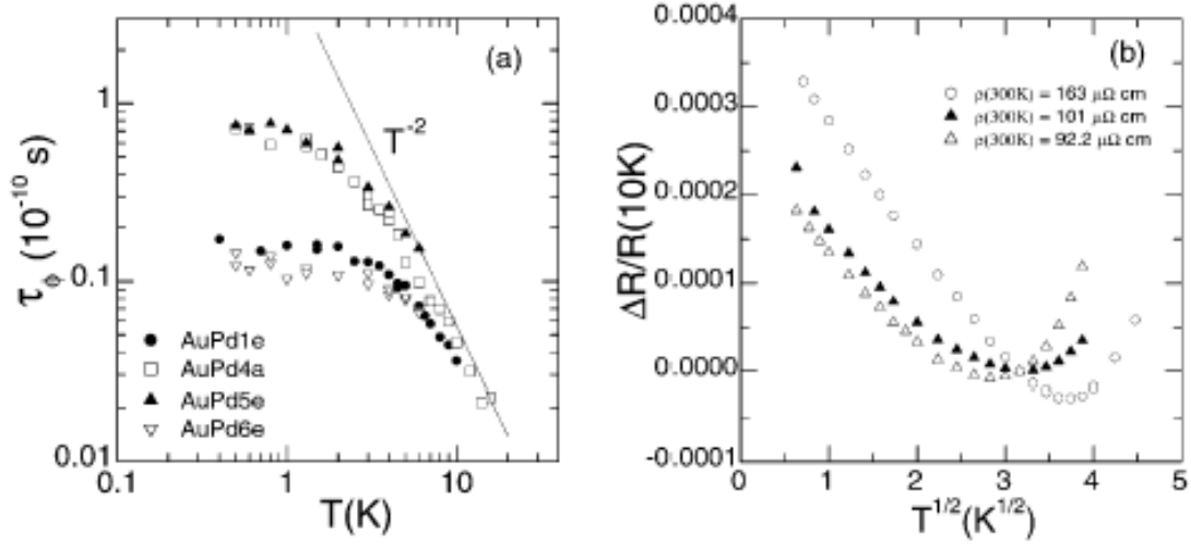
Fig. 1 – (a) \tau_\phi as a function of temperature for four as-prepared AuPd thick films. (b) \Delta R/R(T) = [R(T) - R(10\text{ K})]/R(10\text{ K}) as a function of \sqrt{T} for three AuPd thick films.
