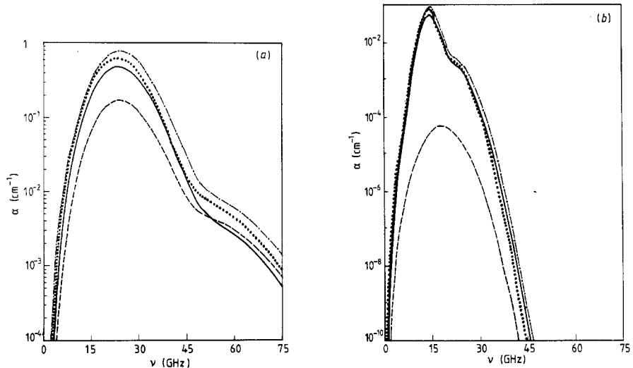
Figure 7. Amplification coefficient of acoustic waves for TR mode as a function of frequency in bismuth films with x = 100 ( E = 1.42 \text{ V cm}^{-1} ) at (a) T = 77 \text{ K} and (b) T = 4.2 \text{ K} : (—) MNENP model; (---) NENP model; (- · - · -) ENP model; (· · · ·) EP model.
