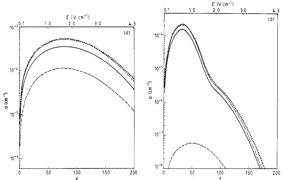
Figure 6. Amplification coefficient of acoustic waves for SV-P mode versus drift parameter x or applied electric field E in bismuth films with \nu = 3 \text{ GHz} at (a) T = 77 \text{ K} and (b) T = 4.2 \text{ K} : (—) MNENP model; (---) NENP model; (- · - · -) ENP model; (· · · ·) EP model.
