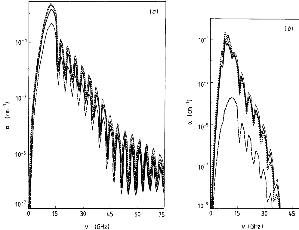
Figure 3. Amplification coefficient of acoustic waves for P-SV mode as a function of frequency in bismuth films with x = 100 ( E = 2 \text{ V cm}^{-1} ) at (a) T = 77 \text{ K} and (b) T = 4.2 \text{ K} : (—) MNENP model; (---) NENP model; (-·-·-) ENP model; (····) EP model.
