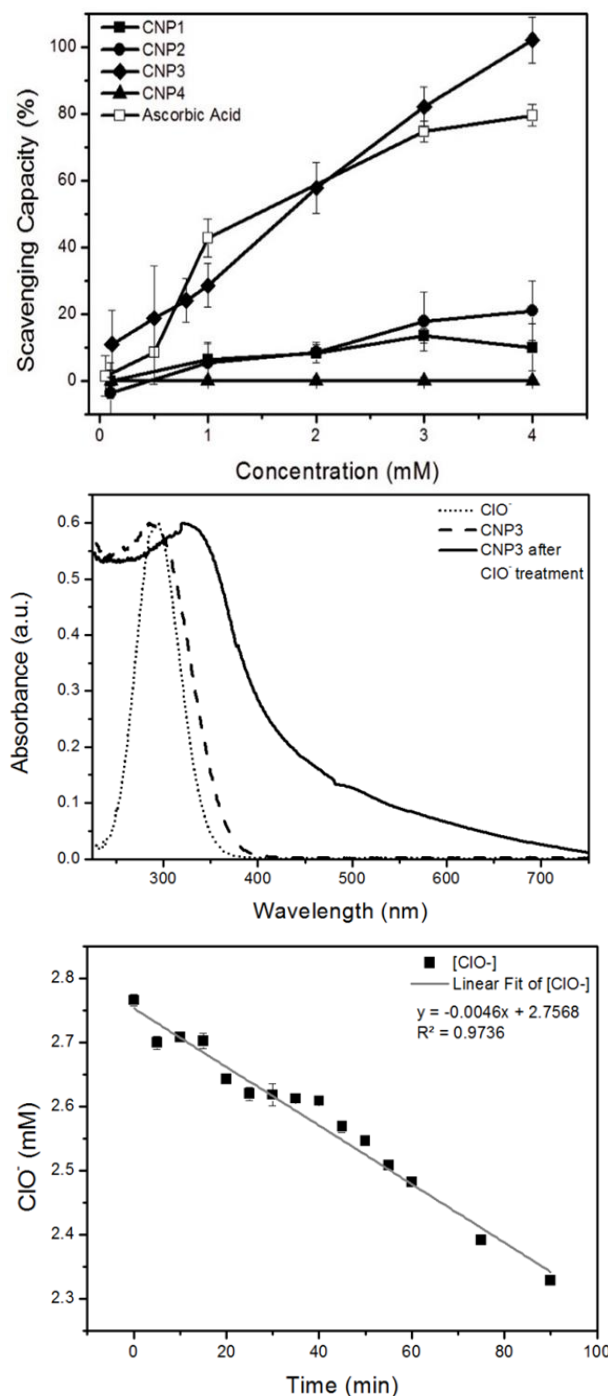
Kinetics of \text{ClO}^- depletion by CNP3
