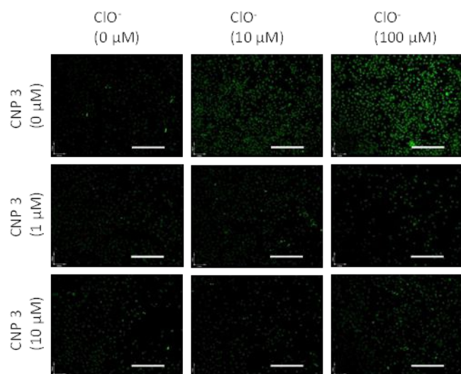
Figure 4. Scavenging of \text{ClO}^- by CNP3 in vitro RAW cell culture model. Pretreatment with 1 \mu\text{M} CNP3 able to scavenge the most of the \text{ClO}^- (comparable to control); scale bar 50 \mu\text{m} .
