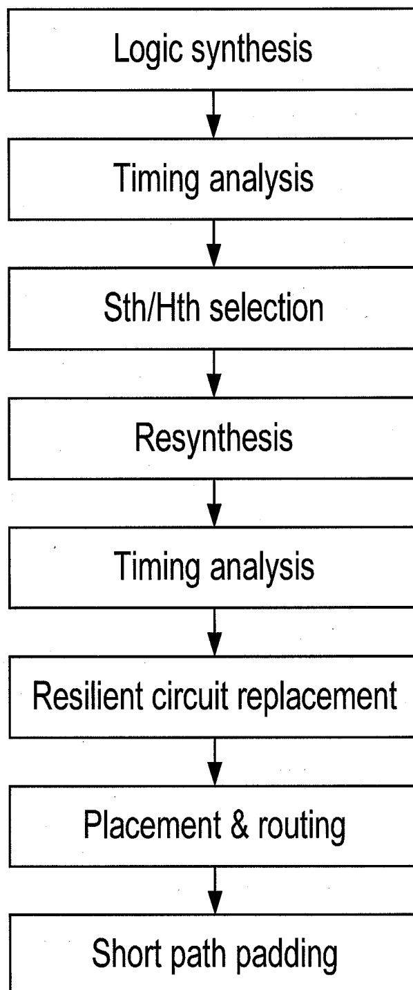
FIG. 2 (Prior Art)
