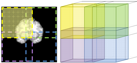
Fig. 10. Demonstration the unit of graph cut at level 1. The region surrounded by yellow, purple, green, and blue dotted line are the unit of graph cut, individually. Each unit perform graph cut once. The left image of this figure is the view in 2-D and the right one is the view in 3-D.
