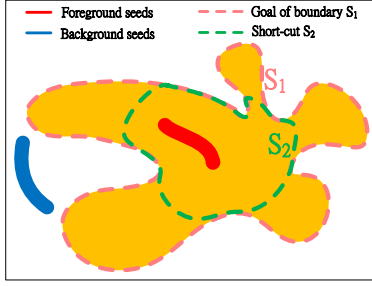
Fig. 1. Short-cut problem of graph cuts. S_1 is the goal of boundary and S_2 is the short-cut path. Although the edge weights of n-links on the goal of boundary S_1 are smaller than those on the short-cut path S_2 , however, the boundary S_1 is too long cause the cost is bigger than short-cut S_2 . Therefore, graph cuts may result in short-cut S_2 instead of boundary S_1 .
