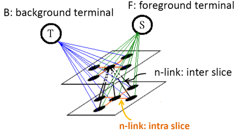
Fig. 7. Demonstration of n-link and t-link. Blue lines are the t-link connecting to background terminal. Green lines are the t-link connecting to foreground terminal. Orange lines are the intra slice n-link (link in the same slice). Black lines are the inter slice n-link (link in different slices).
