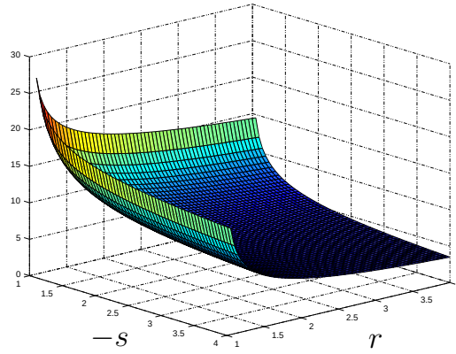
Figure 4.4. The period function T_0(r, 2, s) with b = 0 .
