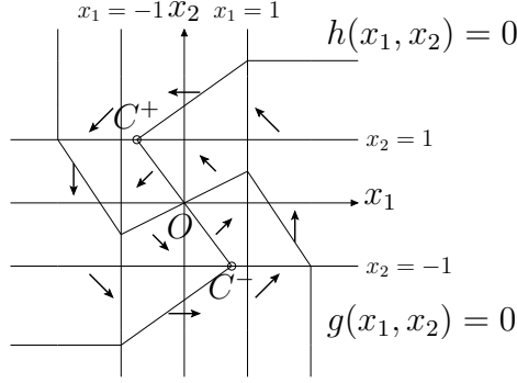
Figure 2.1. Isoclines and vector fields of system (1.1) when b = 0 .
