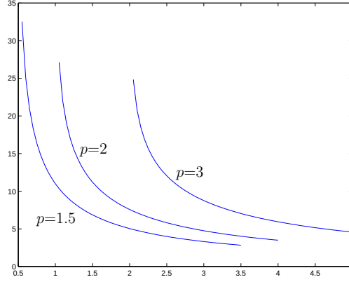
Figure 4.3. The period function T_0(r, p, -r) with b = 0 .
