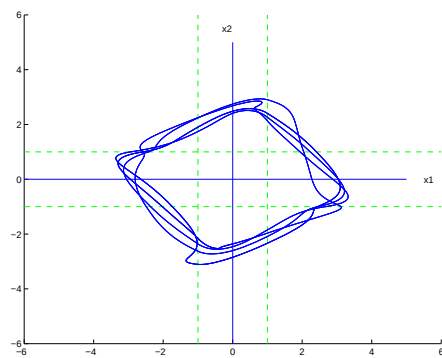
(b) b = 0.78, T_b = \frac{15}{4}T
