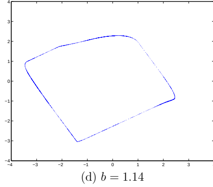
Figure 5.3. Some typical quasi-periodic orbit (a) and (c) and their \omega -limit set \hat{\omega} of the Poincaré map (b) and (d), A = [1.2, 2, -1.2] and T = 4 .
