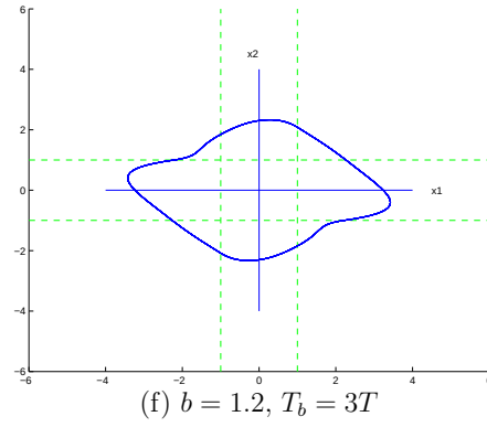
Figure 5.2. Some typical orbits in B_{m,n} prior to chaotic regions, A = [1.2, 2, -1.2] and T = 4 .
