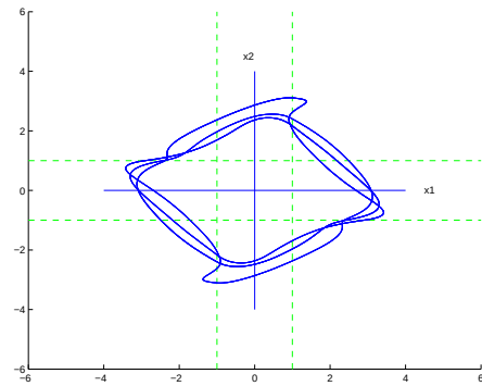
(c) b = 0.9, T_b = \frac{11}{3}T
