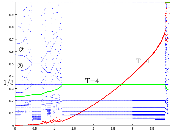
Figure 3.1. FFT of the largest 20 modes for the ZN-case : A = [1.2, 2, -1.2] and T = 4 .
