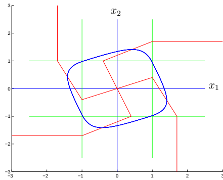
(b) A = [0.5, 1.2, -0.5] , b = 0
