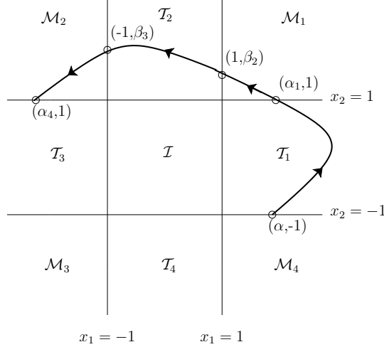
Figure 4.1. A typical orbit of (1.1) with initial condition (\alpha, -1) , and 1 \leq \alpha \leq p - s .
