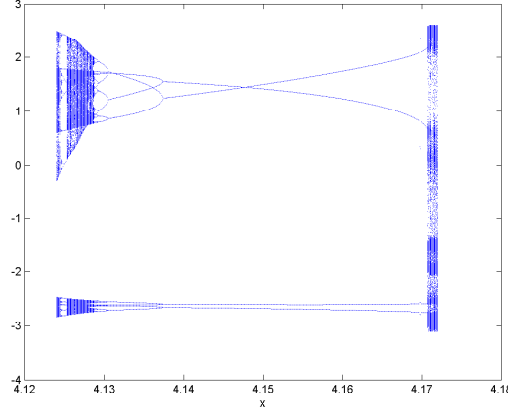
Figure 7.3. Bifurcations diagram for ZN-case with b in window W_4 = (4.124, 4.172) .
