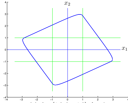
(a) A = [1.2, 2, -1.2] , b = 0
