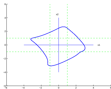
(a) b = 0.5, T_b = 4T
