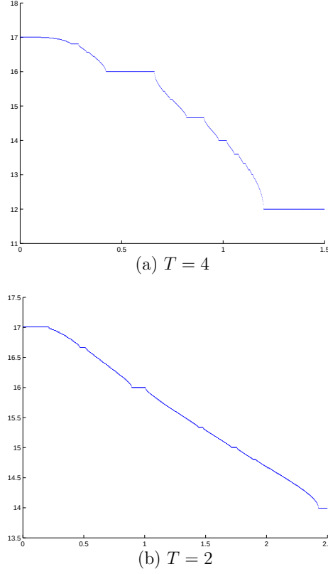
Figure 5.1. Devil's staircase like period function T_b , A = [1.2, 2, -1.2] , (a) T = 4 and (b) T = 2 .
