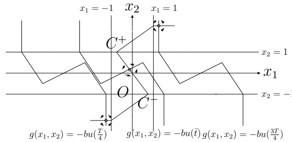
Figure 2.2. Isoclines and vector fields for b > 0 .
