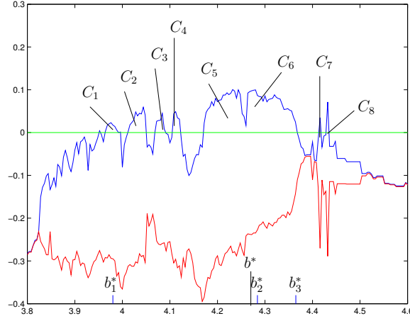
Figure 7.1. Lyapunov exponents diagram for the ZN-case with b in (3.8, 4.6) , b_1^* = 3.98 , b_2^* = 4.284 , b_3^* = 4.365 and b^* = 4.2697 .
