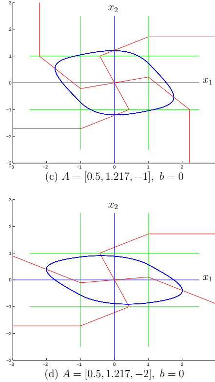
Figure 4.2. Typical limit cycles of (1.1) with b = 0 , (a) exterior cycle, (b)~(d) non-exterior cycles.
