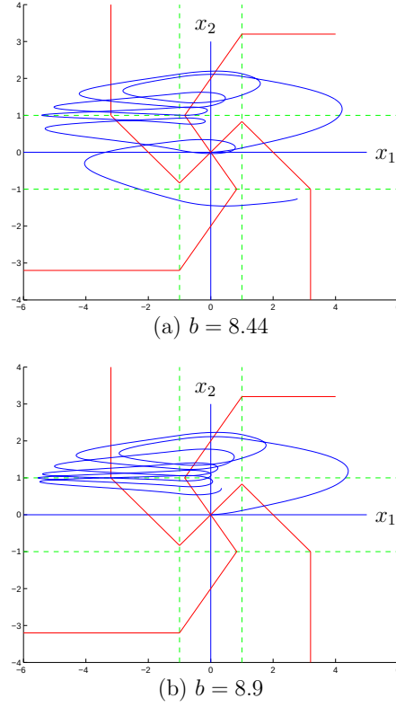
Figure 3.3 Critical trajectories can circle around C^+ or C^- many times when A = [1.2, 2, -1.2] and T = 2 .
