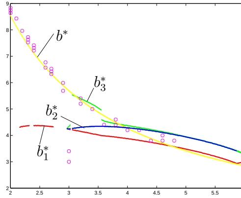
Figure 7.5. Critical numbers b^* , b_k^* , k = 1, 2, 3 for varying T , A = [1.2, 2, -1.2] .
