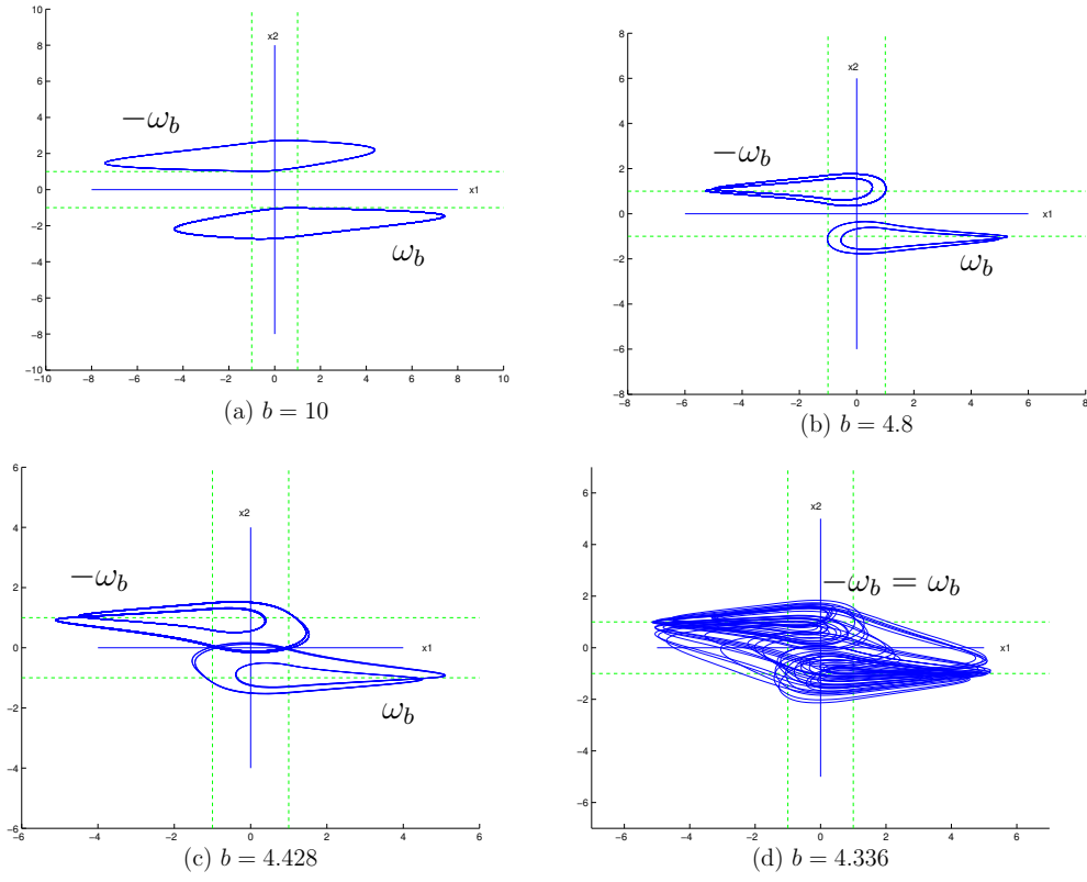
Figure 6.1. Crises induced by \omega_b and -\omega_b when A = [1.2, 2, -1.2] and T = 4 .
