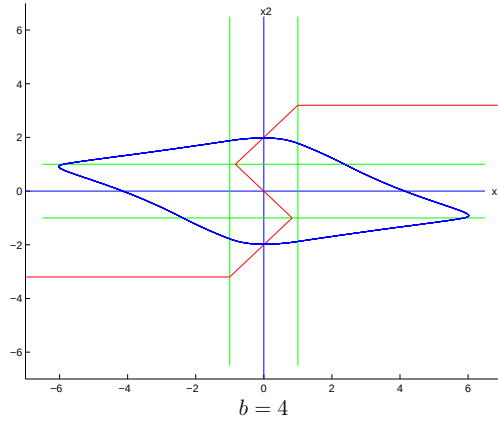
Figure 6.2. \omega_b = -\omega_b when A = [1.2, 2, -1.2] and T = 10 .
