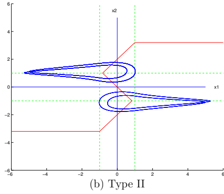
Figure 7.2. (a) Type I: the orbit \Gamma_b circles around all three points C^+ , O and C^- . (b) Type II: the orbit \Gamma_b does not circle around all of three points C^+ , O and C^- .
