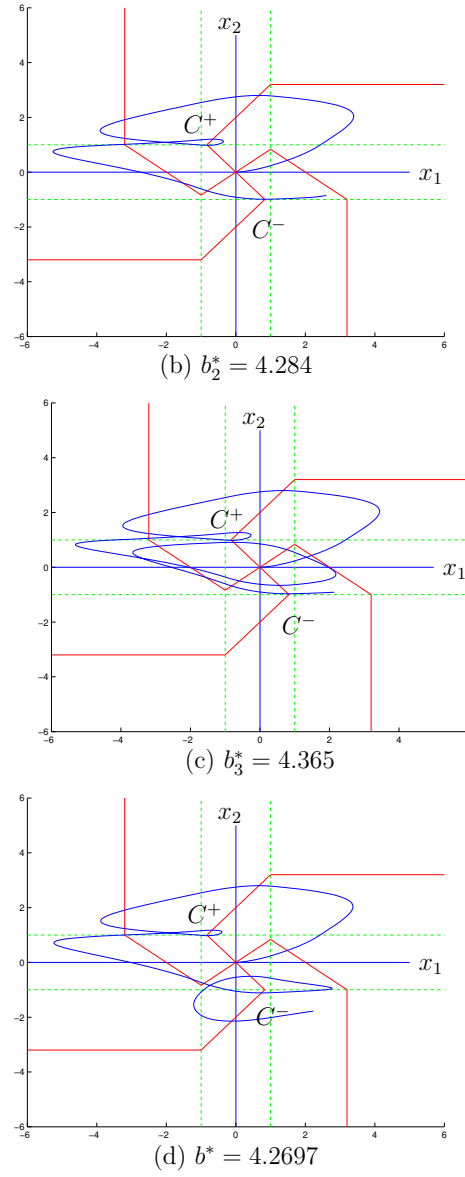
Figure 3.2 Critical trajectories of b_1^* , b_2^* , b_3^* and b^* , when A = [1.2, 2, -1.2] and T = 4 .
