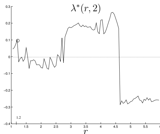
Figure 7.7. The maximum Lyapunov exponent function \lambda^*(r, 2) for A = [r, 2, -r] .
