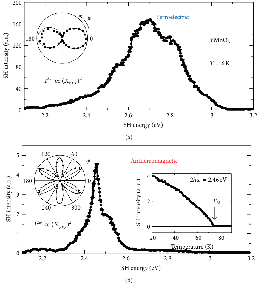
FIGURE 6: SHG spectra of \text{YMnO}_3 due to (a) the ferroelectric ordering and (b) antiferromagnetic ordering; inset: temperature dependence of the SHG intensity of 2.46 eV [34]. Reprinted figure with permission from Fröhlich et al. [34]. Copyright (1998) by the American Physical Society.
