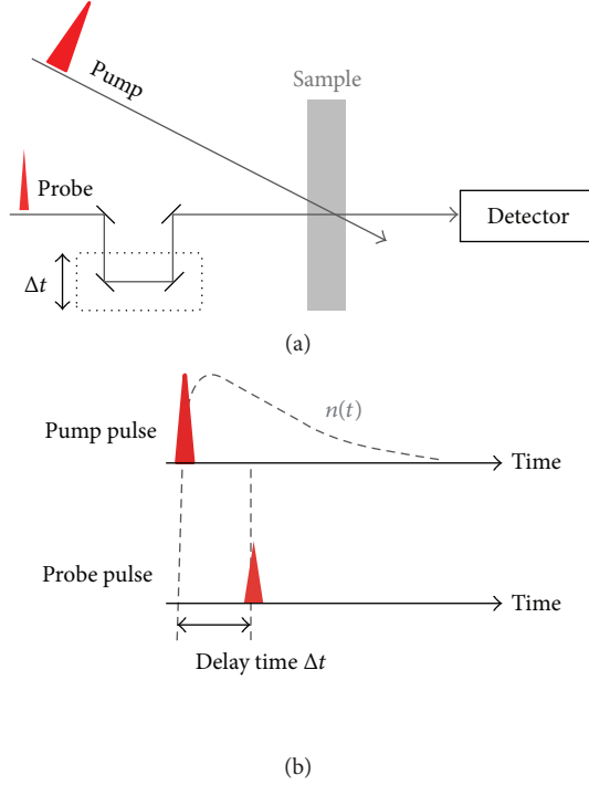
FIGURE 7: (a) Schematic diagram of pump-probe technique. Time delay ( \Delta t ) between pump and probe pulses can be controlled by a mechanical delay line. (b) The fundamental principle of pump-probe experiments. Time varying refractive index n(t) changes of the sample induced by pump pulses were observed by detecting the intensity variations of probe pulses.
