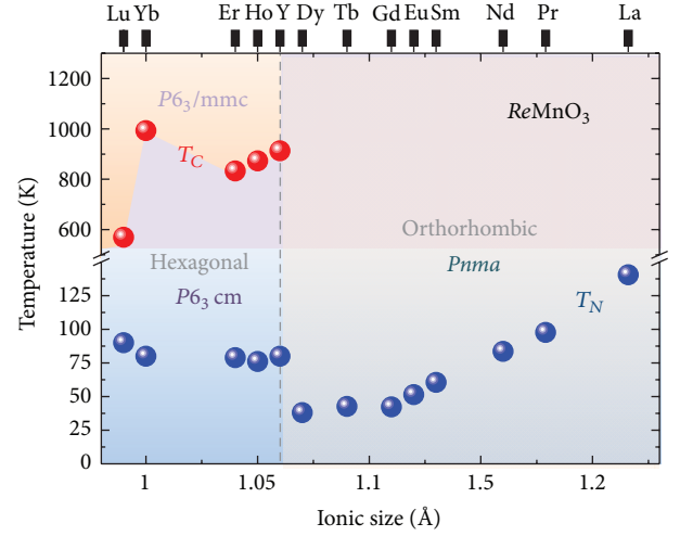
FIGURE 1: Lattice structure in \text{ReMnO}_3 as a function of the size of the rare-earth elements [11, 24–29].
