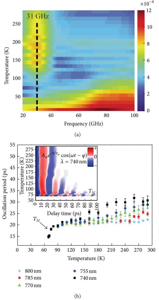
FIGURE 11: (a) Fourier transform amplitudes for coherent oscillation of \text{YMnO}_3 [39]. Reprinted with permission from Jang et al. [39]. Copyright 2010, American Institute of Physics. (b) Temperature dependence oscillation period in \Delta R/R at various wavelengths of \text{HoMnO}_3 . Inset: the evolution of the oscillation component in \Delta R/R at various temperatures [38]. Figures were reproduced with permission from Shih et al. [38].
