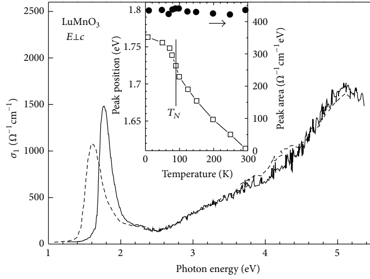
FIGURE 3: Electronic conductivity of \text{LuMnO}_3 at 300 K (dashed line) and 10 K (solid line). Inset: temperature-dependent peak position (open squares) and spectral weight (solid circles) of the absorption peak around 1.7 eV [31]. Reprinted figure with permission from Souchkov et al. [31]. Copyright (2003) by the American Physical Society.
