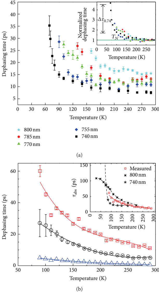
FIGURE 10: (a) Temperature dependence dephasing time of the oscillation component in \Delta R/R at various wavelengths of \text{HoMnO}_3 . Inset: the normalized dephasing time as a function of temperatures at various wavelengths [38]. Figures were reproduced with permission from Shih et al. [38]. (b) Temperature dependence of dephasing times: red squares for acoustic phonons, black circles for optical phonons, and blue triangles for electronic relaxation time [37]. Figures were reproduced with permission from Jang et al. [37].
