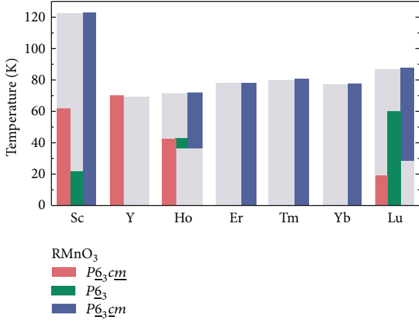
FIGURE 5: Magnetic symmetry of the hexagonal manganites. Sc, Ho, and Lu show a coexistence of magnetic phases with temperature intervals being sample specific. (Rare-earth spin ordering below 6 K was not considered) [33]. Reprinted figure with permission from Fiebig et al. [33]. Copyright (2000) by the American Physical Society.
