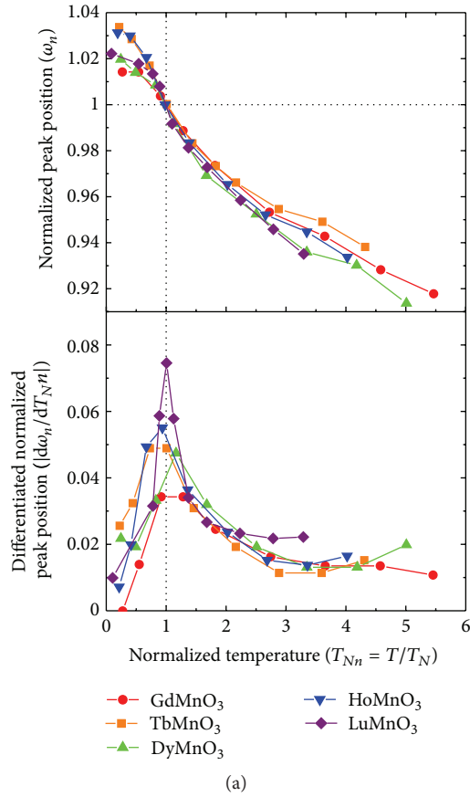
FIGURE 4: (a) Upper panel: temperature dependence of the peak positions normalized to the peak position at T_N as a function of the normalized temperature T_{Nn} (\equiv T/T_N) . Lower panel: absolute value of normalized peak position differentiated to normalized temperature [32]. Reprinted figure with permission from Choi et al. [32]. Copyright (2008) by the American Physical Society. (b) Schematic diagram of the d-d transition in \text{ReMnO}_3 . The red arrows indicate electrons reside in the d orbitals, and the gray arrow indicates lowering of e_{2g} band caused by the temperature reduction.
