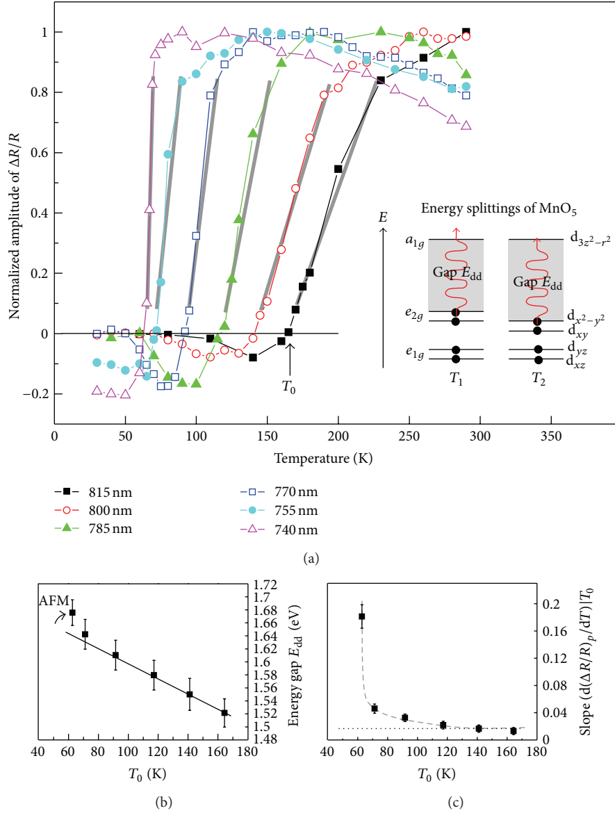
FIGURE 8: (a) Normalized amplitude of \Delta R/R as a function of temperature at various wavelengths. The insets illustrate splitting of the \text{Mn}^{3+} energy levels in the local environment \text{MnO}_5 for photon energy above and below E_{dd} ( T_1 > T_2 ). (b) Energy gap E_{dd} as a function of T_0 . E_{dd} is estimated from the wavelengths in (a). The dashed line emphasizes linear behavior in the high-temperature range. (c) The slope of temperature-dependent normalized amplitude of \Delta R/R in (a) (gray thick lines) as a function of T_0 at various wavelengths. The dashed line emphasizes behavior of the slope [35]. Reprinted figure with permission from Shih et al. [35]. Copyright (2009) by the American Physical Society.
