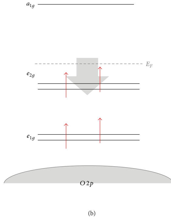
FIGURE 4: (a) Upper panel: temperature dependence of the peak positions normalized to the peak position at T_N as a function of the normalized temperature T_{Nn} (\equiv T/T_N) . Lower panel: absolute value of normalized peak position differentiated to normalized temperature [32]. Reprinted figure with permission from Choi et al. [32]. Copyright (2008) by the American Physical Society. (b) Schematic diagram of the d-d transition in \text{ReMnO}_3 . The red arrows indicate electrons reside in the d orbitals, and the gray arrow indicates lowering of e_{2g} band caused by the temperature reduction.
