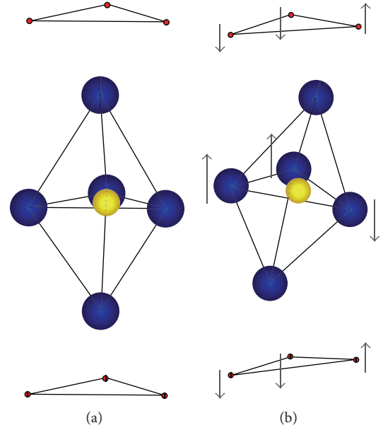
FIGURE 2: Schematic of \text{MnO}_5 bipyramid above and below T_C , respectively. (a) Centrosymmetric structure with space group P6_3/mmc and (b) noncentrosymmetric with P6_3cm space group. The arrows indicate atomic displacements with respect to the centrosymmetric structure [14, 30]. (Red: Re, blue: O, yellow: Mn).
