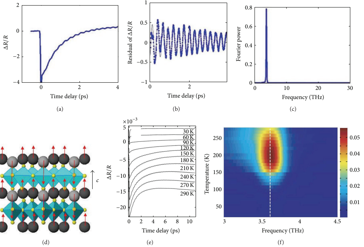
FIGURE 9: LuMnO 3 measured at 293 K. (a) \Delta R/R as a function of time delay. (b) Oscillation component after subtraction of the slowly varying response. (c) Fourier power spectrum of the data with frequency 3.61 THz. (d) Schematic of the coherently excited A 1 phonon mode [36]. Reprinted figure with permission from Lou et al. [36]. Copyright (2009) by the American Physical Society. (e) \Delta R/R at various temperatures. (f) Fourier transformed amplitudes of coherent optical phonon [37]. Figures were reproduced with permission from Jang et al. [37].
