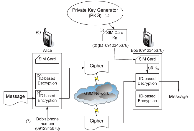
Fig. 2. ID-based End-to-end Encryption System
