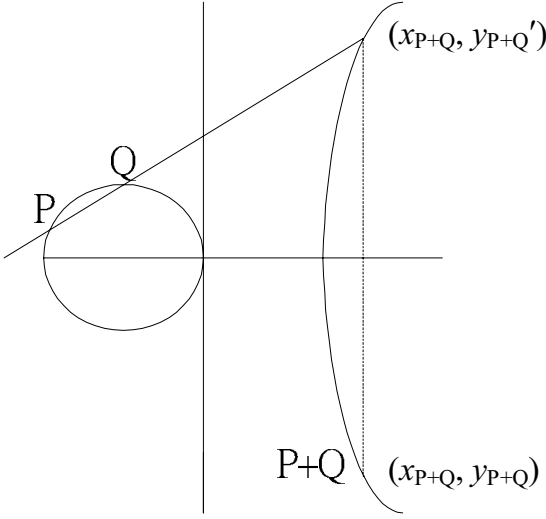
Fig. 1. Group law on an elliptic curve
